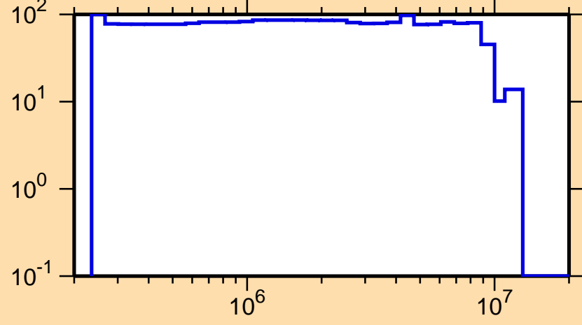
\Delta\sigma/\sigma vs. E for ^{242}\text{Bk}(n,n_1)
