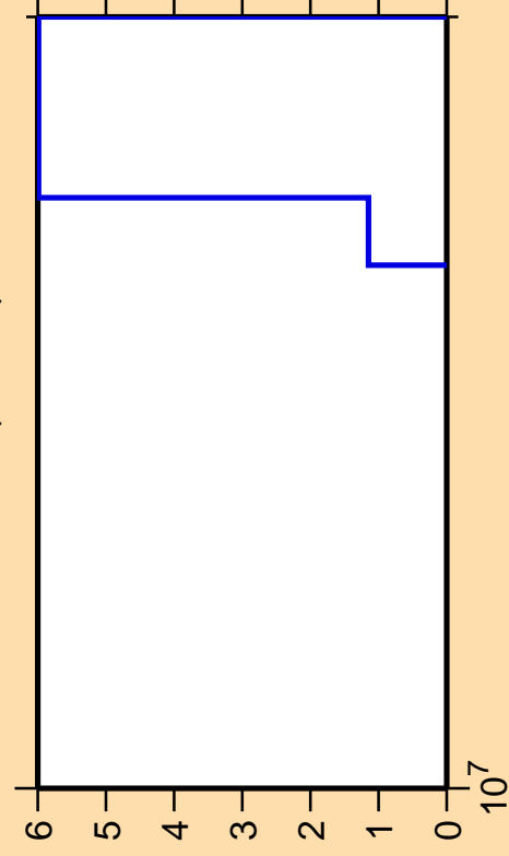
\Delta\sigma/\sigma vs. E for ^{242}\text{Bk} (mt 45)
