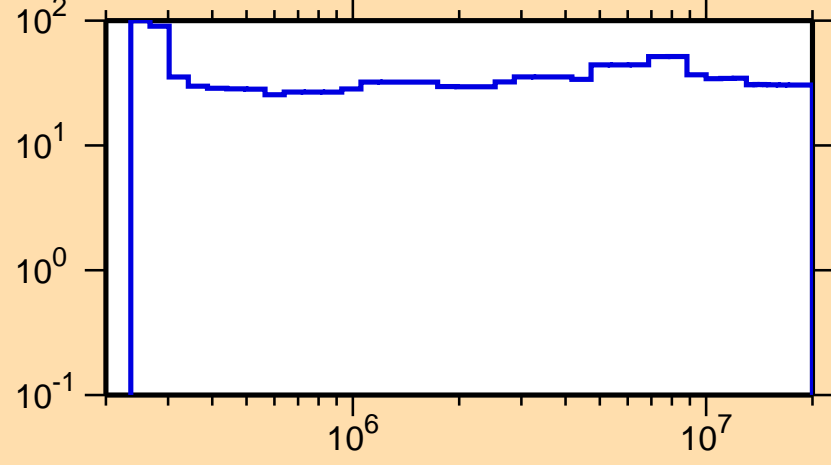
\Delta\sigma/\sigma vs. E for ^{242}\text{Bk}(n,\text{inel.})
