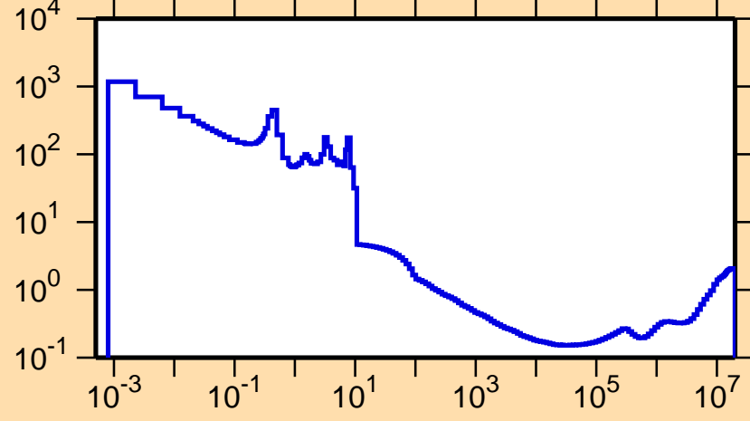
\sigma vs. E for ^{242}\text{Bk}(n,f)
