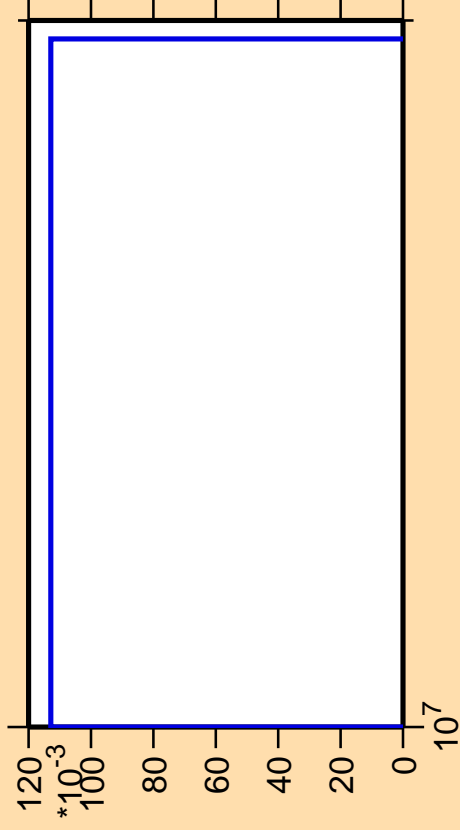
\Delta\sigma/\sigma vs. E for ^{242}\text{Bk} (mt 45)
