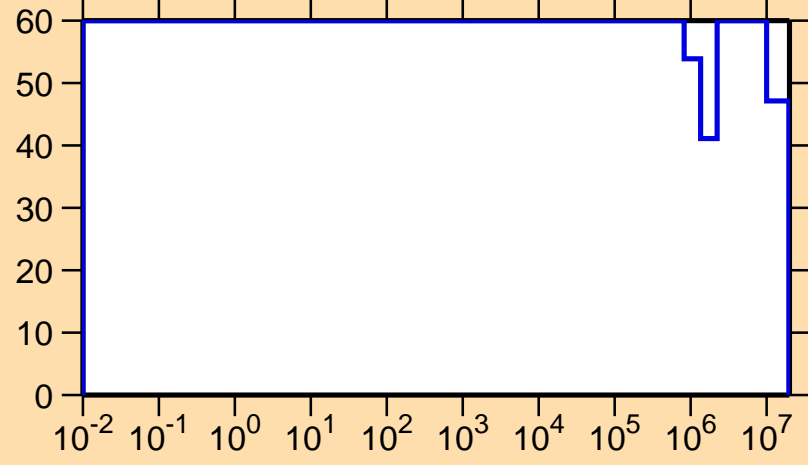
\Delta\sigma/\sigma vs. E for ^{242}\text{Bk}(n,p)
