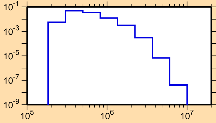
\sigma vs. E for ^{242}\text{Bk}(n,n_1)
