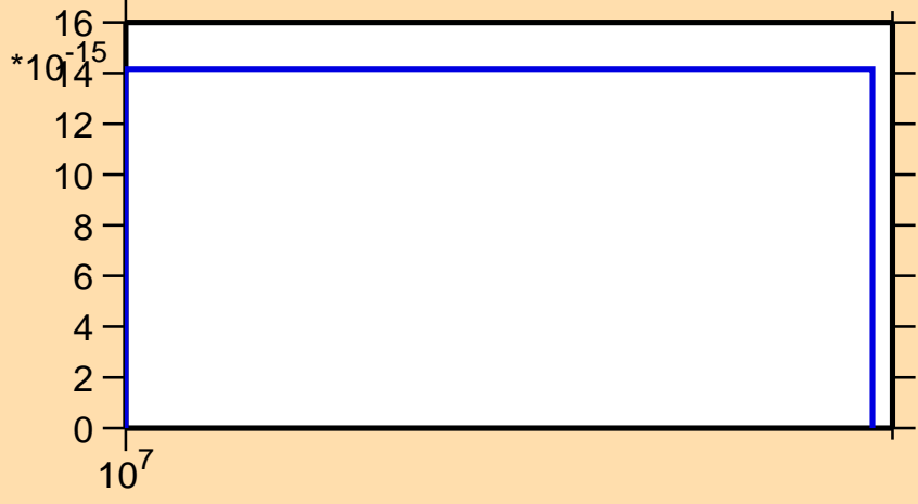
\sigma vs. E for ^{242}\text{Bk} (mt 34)
