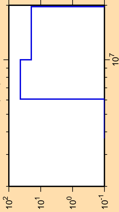
\Delta\sigma/\sigma vs. E for ^{242}\text{Bk}(n,d)
