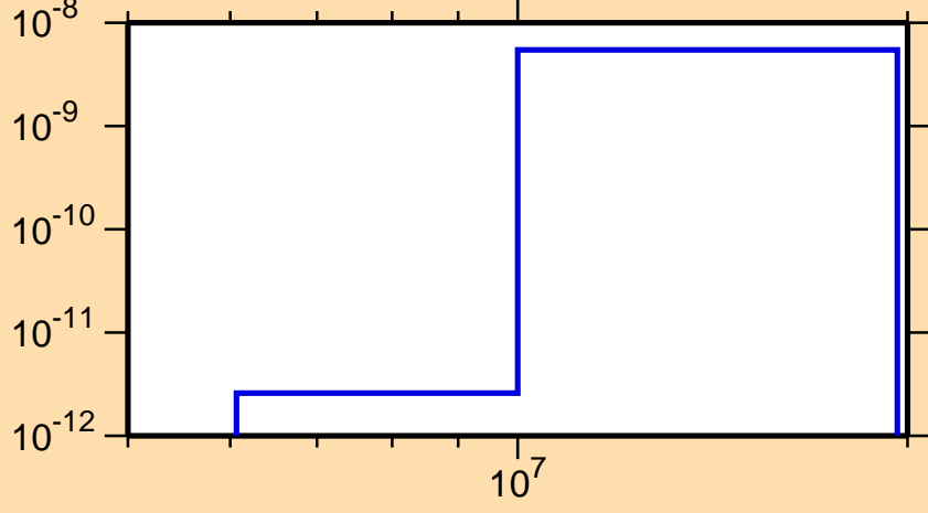
\sigma vs. E for ^{242}\text{Bk}(n,2n\alpha)
