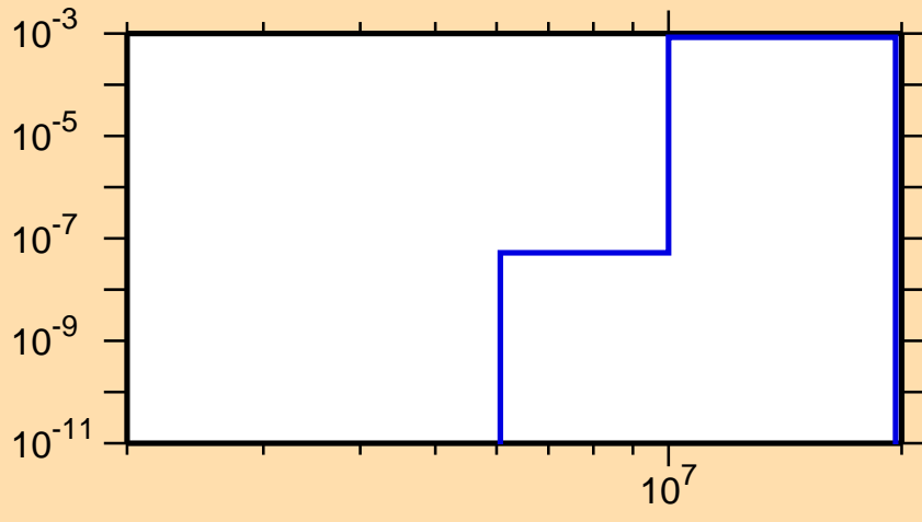
\sigma vs. E for ^{242}\text{Bk}(n,d)
