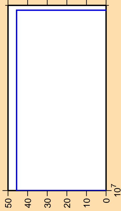
\Delta\sigma/\sigma vs. E for ^{242}\text{Bk}(n,nd)
