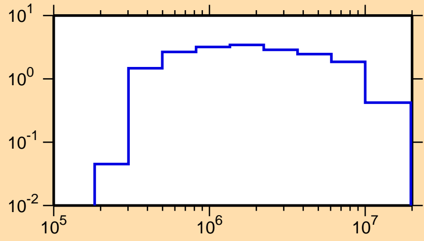
\sigma vs. E for ^{242}\text{Bk}(n,\text{inel.})
