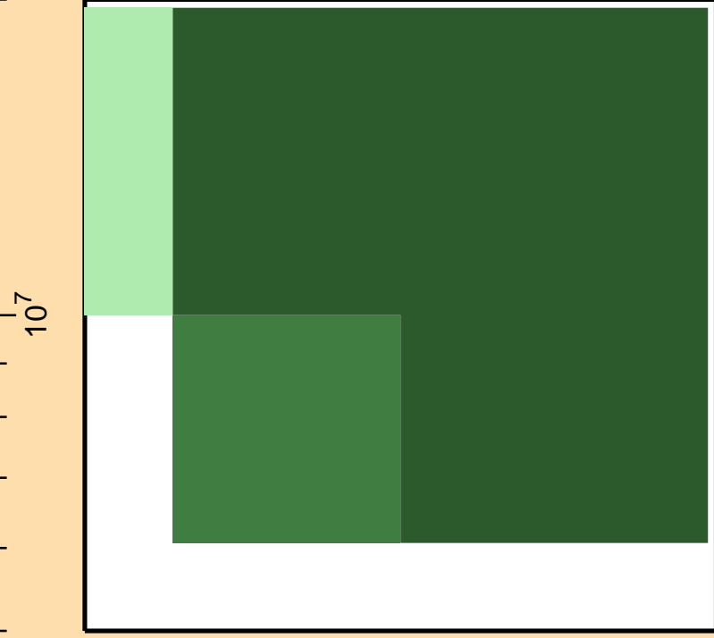
\Delta\sigma/\sigma vs. E for ^{242}\text{Bk}(n,\text{inel.})
