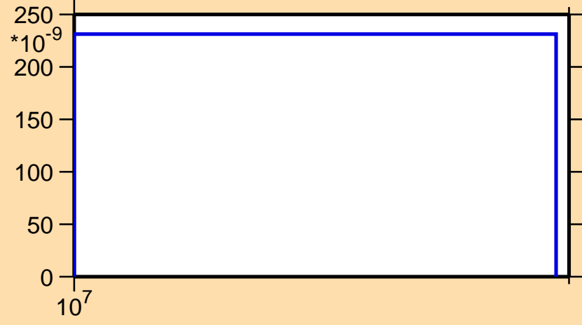
\sigma vs. E for ^{242}\text{Bk}(n,nd)
