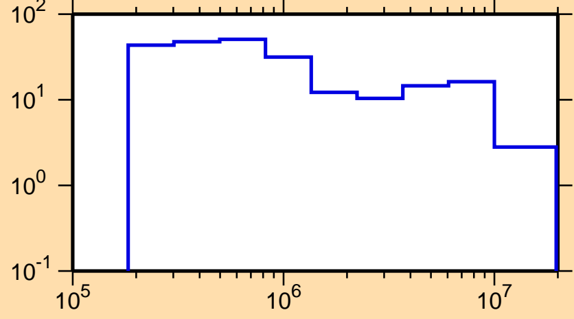
\Delta\sigma/\sigma vs. E for ^{242}\text{Bk}(n,\text{el.})
