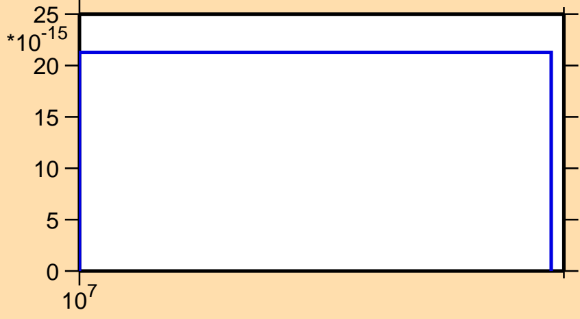
\sigma vs. E for ^{242}\text{Bk} (mt 45)
