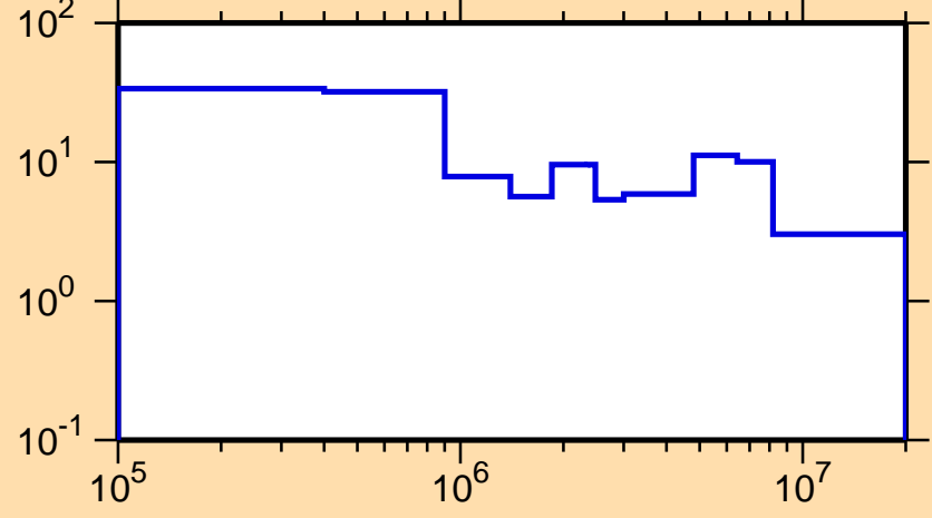
\Delta\sigma/\sigma vs. E for ^{242}\text{Bk}(n,\text{tot.})
