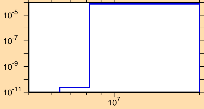
\sigma vs. E for ^{242}\text{Bk}(n,t)
