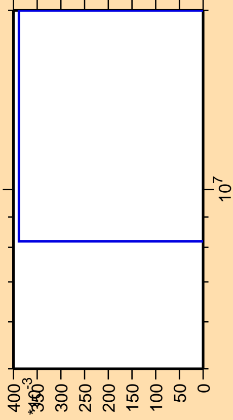
\Delta\sigma/\sigma vs. E for ^{242}\text{Bk}(\text{mt117})
