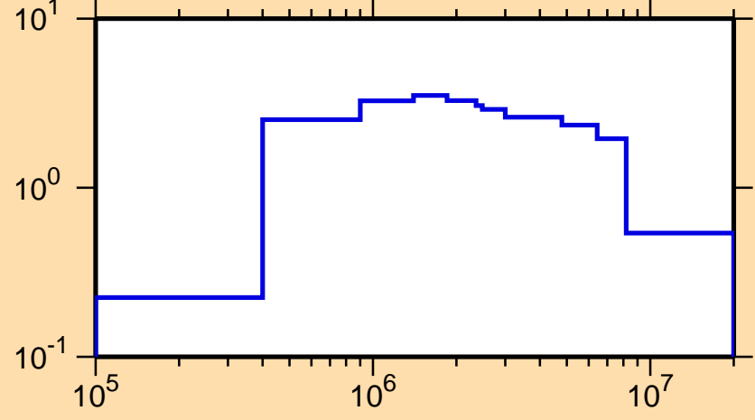
\sigma vs. E for ^{242}\text{Bk}(n,\text{inel.})
