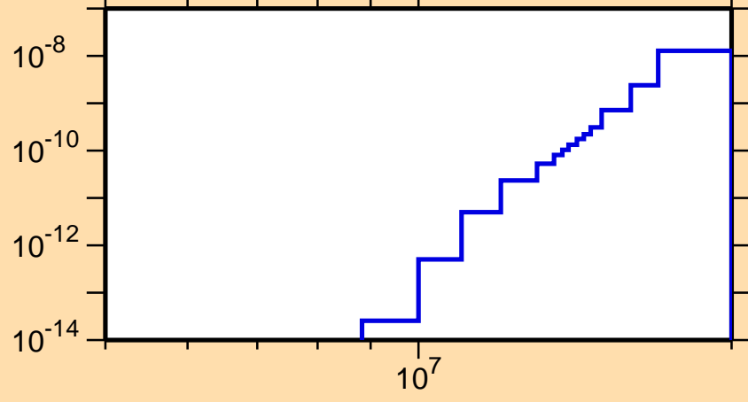
\sigma vs. E for ^{243}\text{Bk}(n,2n\alpha)
