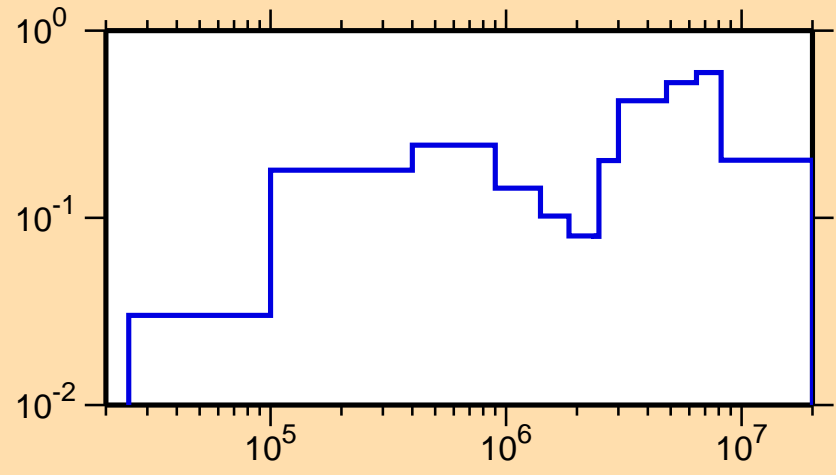
\sigma vs. E for ^{243}\text{Bk}(n,\text{inel.})
