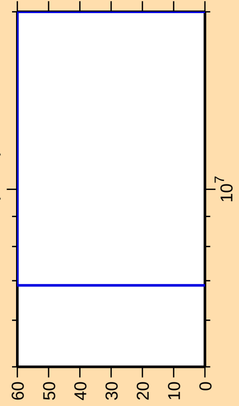
\Delta\sigma/\sigma vs. E for ^{245}\text{Bk}(n,2n)
