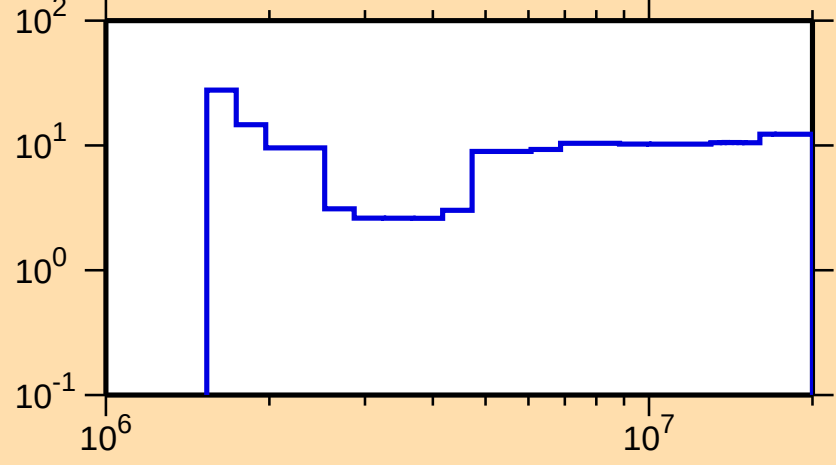
\Delta\sigma/\sigma vs. E for ^{245}\text{Bk}(n,\text{nonel.})
