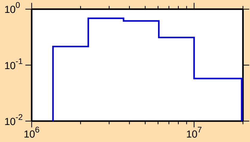
\sigma vs. E for ^{245}\text{Bk}(n,\text{inel.})
