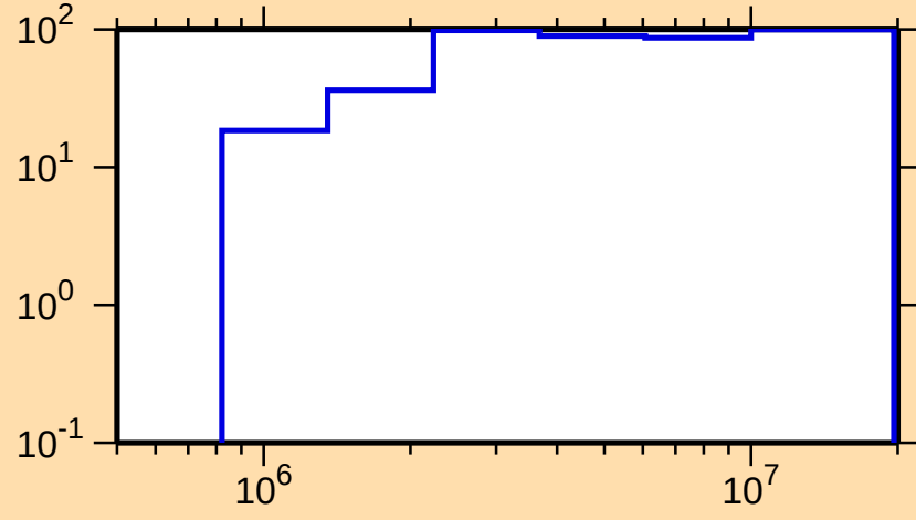
\Delta\sigma/\sigma vs. E for ^{245}\text{Bk}(n,\gamma)
