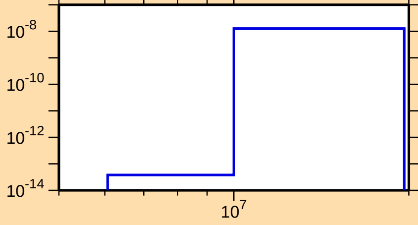
\sigma vs. E for ^{245}\text{Bk}(n,2n\alpha)
