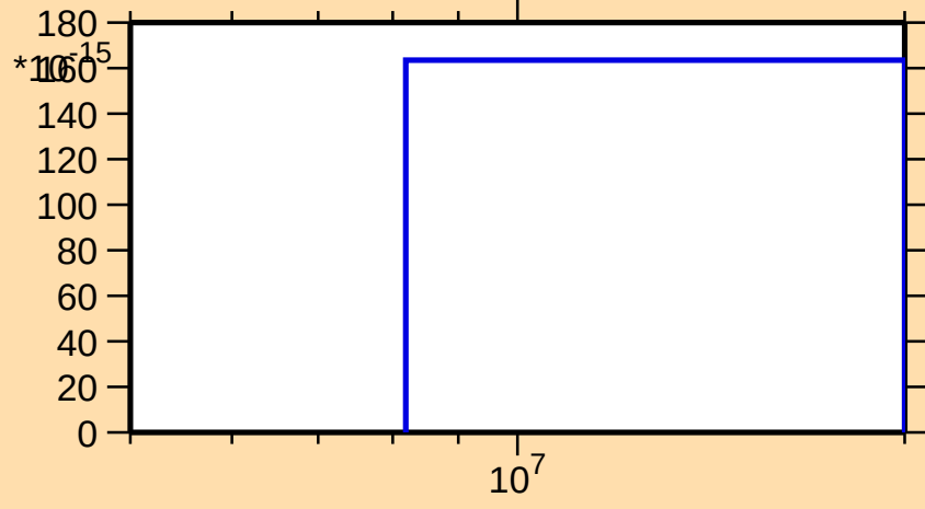
\sigma vs. E for ^{245}\text{Bk}(n,p\alpha)
