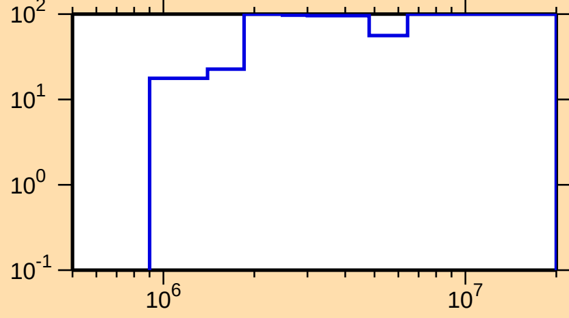
\Delta\sigma/\sigma vs. E for ^{245}\text{Bk}(n,\gamma)
