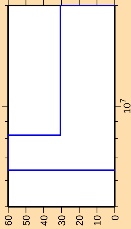
\Delta\sigma/\sigma vs. E for ^{245}\text{Bk}(n,d)
