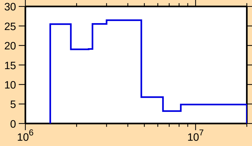
\Delta\sigma/\sigma vs. E for ^{245}\text{Bk}(n,f)
