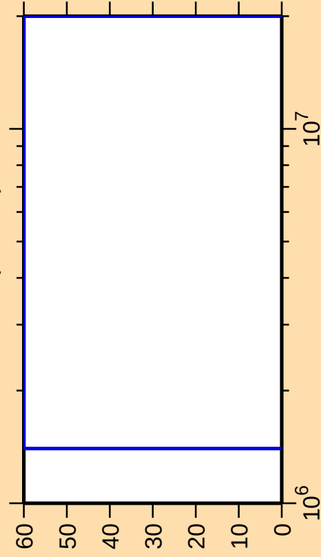
\Delta\sigma/\sigma vs. E for ^{245}\text{Bk}(n,\text{inel.})
