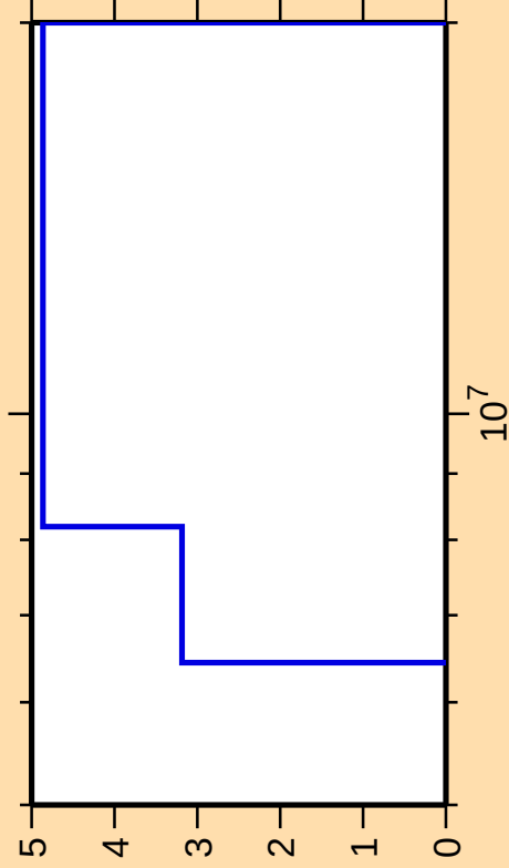
\Delta\sigma/\sigma vs. E for ^{245}\text{Bk}(n,f)
