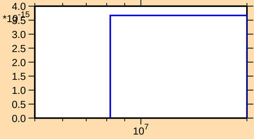
\sigma vs. E for ^{245}\text{Bk}(\text{mt 11})
