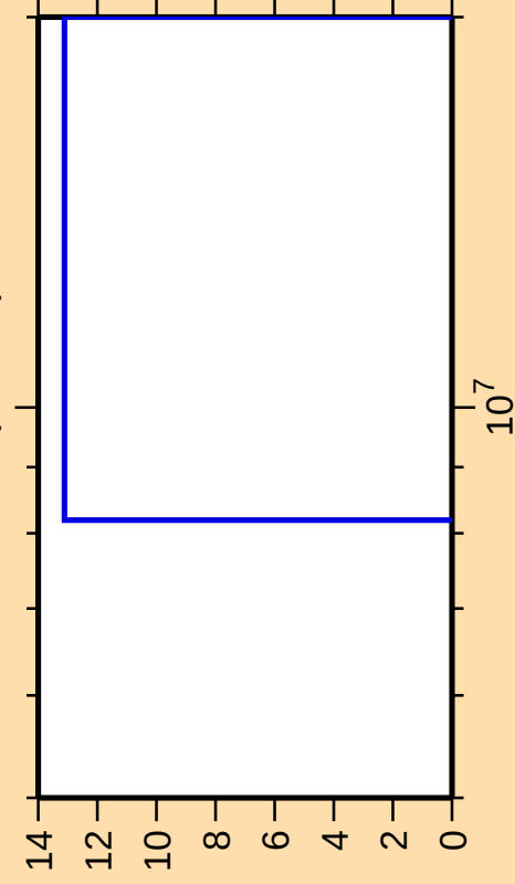
\Delta\sigma/\sigma vs. E for ^{245}\text{Bk}(n,\text{He3})
