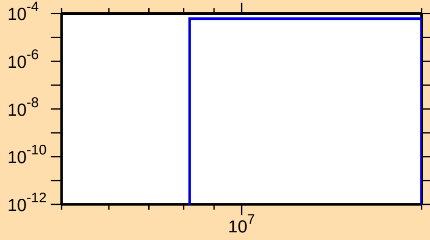
\sigma vs. E for ^{245}\text{Bk}(n,t)
