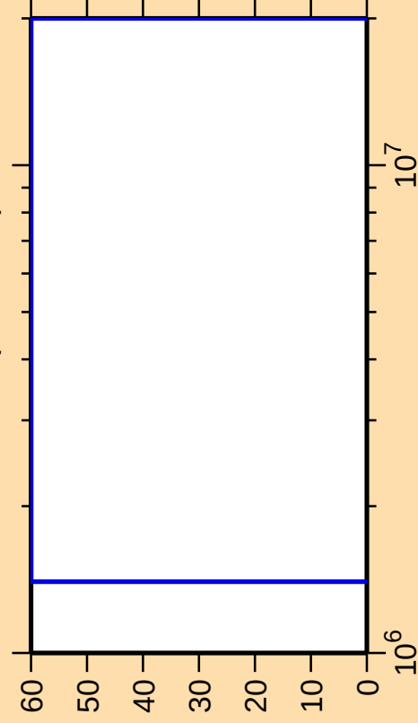
\Delta\sigma/\sigma vs. E for ^{245}\text{Bk}(n,\text{ncont.})
