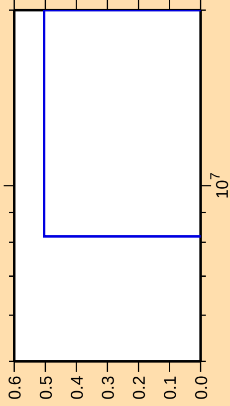
\Delta\sigma/\sigma vs. E for ^{245}\text{Bk}(n,p\alpha)
