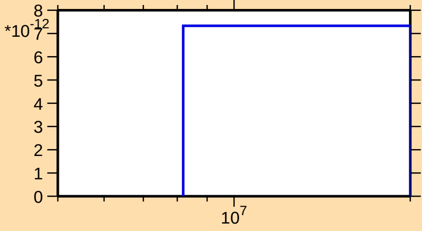
\sigma vs. E for ^{245}\text{Bk}(n,\text{He3})
