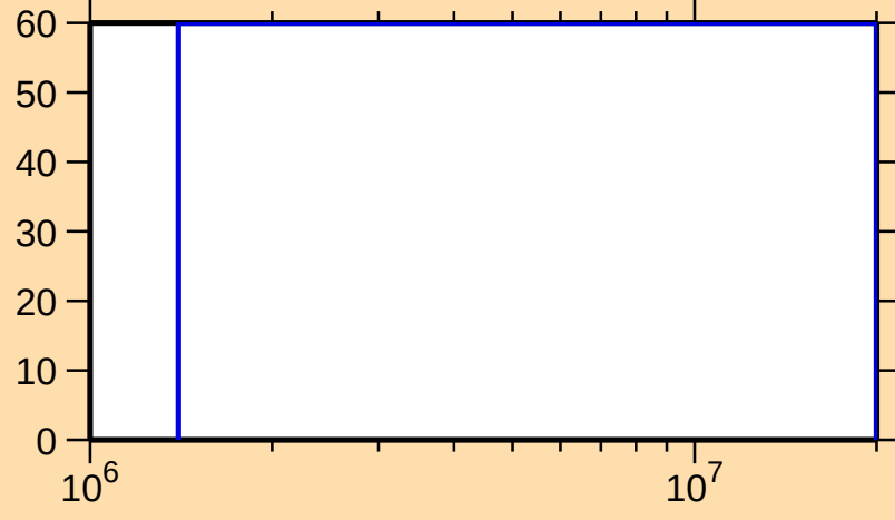
\Delta\sigma/\sigma vs. E for ^{245}\text{Bk}(n,n\text{cont.})
