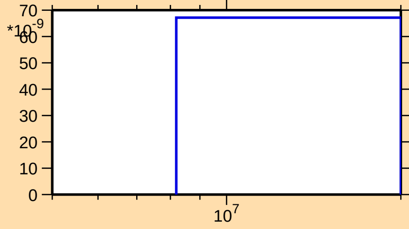
\sigma vs. E for ^{245}\text{Bk}(n,nt)
