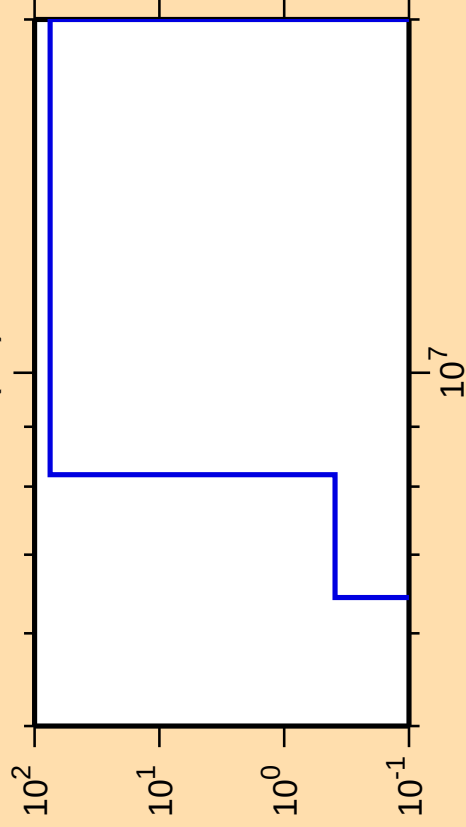
\Delta\sigma/\sigma vs. E for ^{245}\text{Bk}(n,t)
