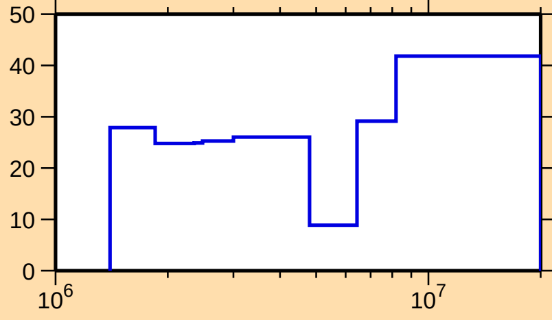
\Delta\sigma/\sigma vs. E for ^{245}\text{Bk}(n,\text{el.})
