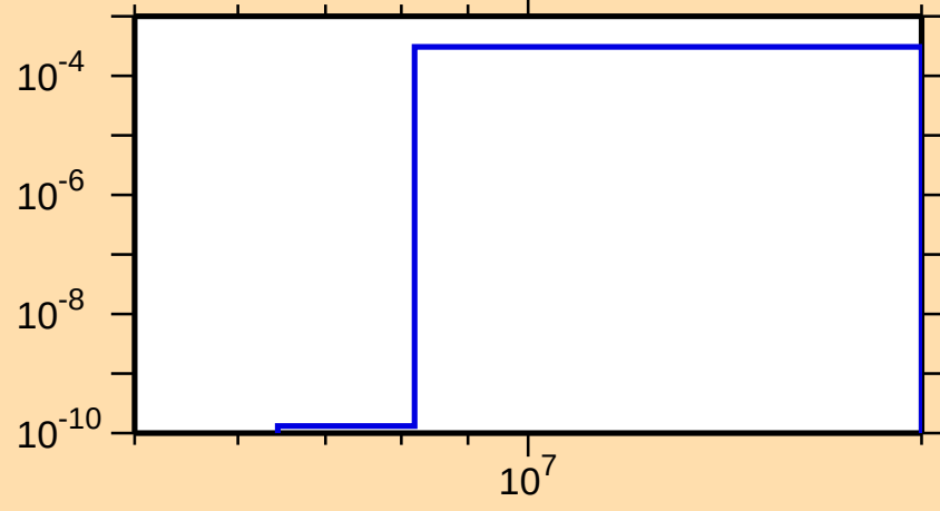
\sigma vs. E for ^{245}\text{Bk}(n,d)
