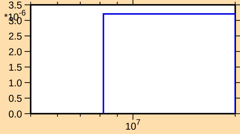
\sigma vs. E for ^{245}\text{Bk}(n,3n\alpha)
