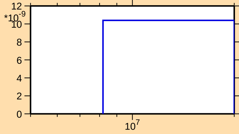
\sigma vs. E for ^{245}\text{Bk}(n,2n\alpha)
