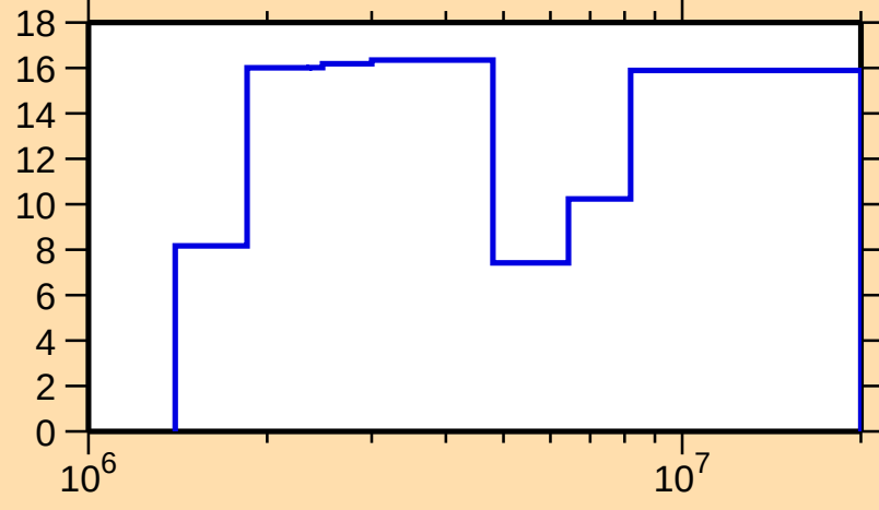
\Delta\sigma/\sigma vs. E for ^{245}\text{Bk}(n,\text{tot.})
