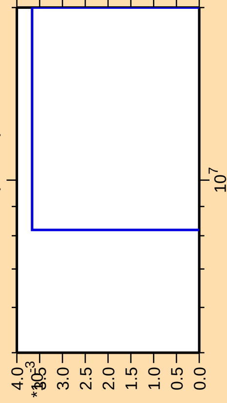
\Delta\sigma/\sigma vs. E for ^{245}\text{Bk}(\text{mt 11})
