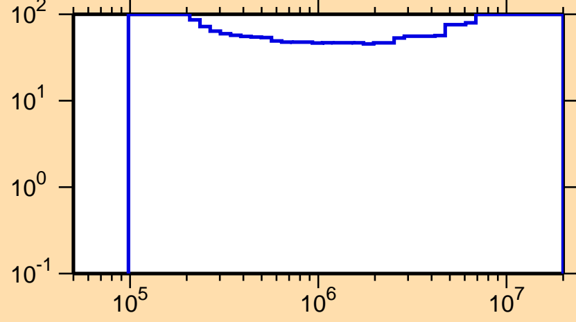
\Delta\sigma/\sigma vs. E for ^{246}\text{Bk}(n,\text{inel.})
