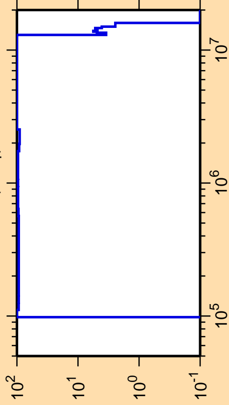
\Delta\sigma/\sigma vs. E for ^{246}\text{Bk}(n,n_1)
