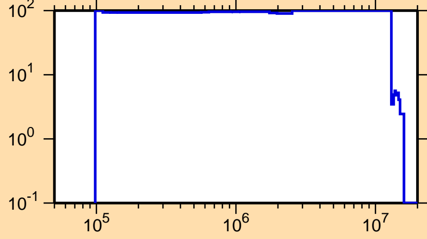
\Delta\sigma/\sigma vs. E for ^{246}\text{Bk}(n,n_1)
