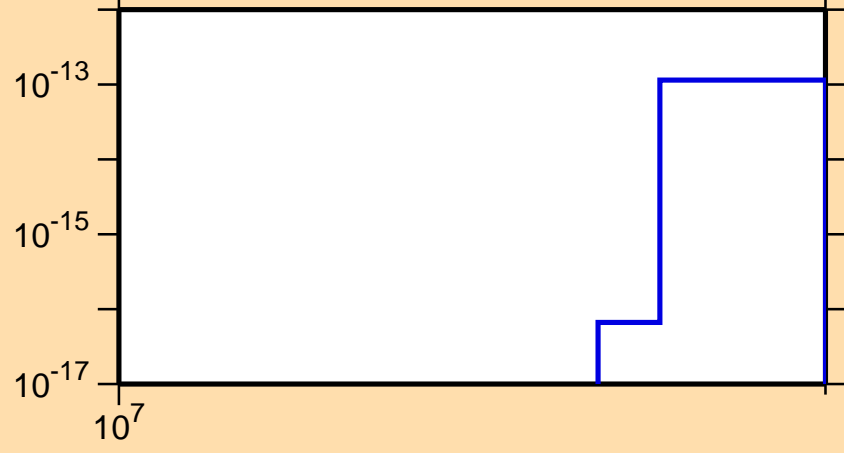
\sigma vs. E for ^{246}\text{Bk} (mt 11)
