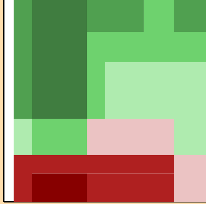
\Delta\sigma/\sigma vs. E for ^{246}\text{Bk}(n,2n)
