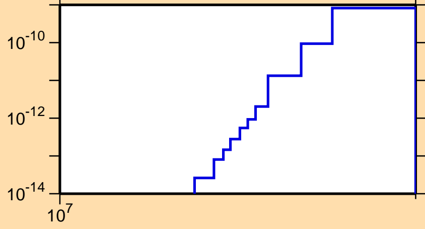
\sigma vs. E for ^{246}\text{Bk}(n,\text{He3})
