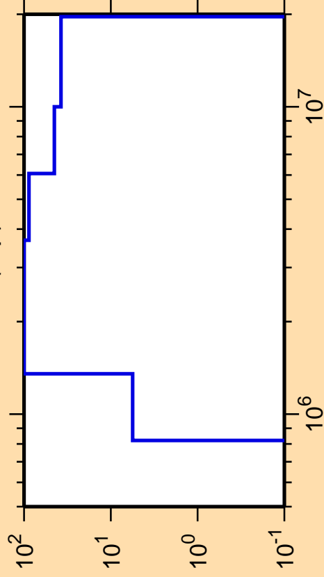
\Delta\sigma/\sigma vs. E for ^{246}\text{Bk}(n,p)
