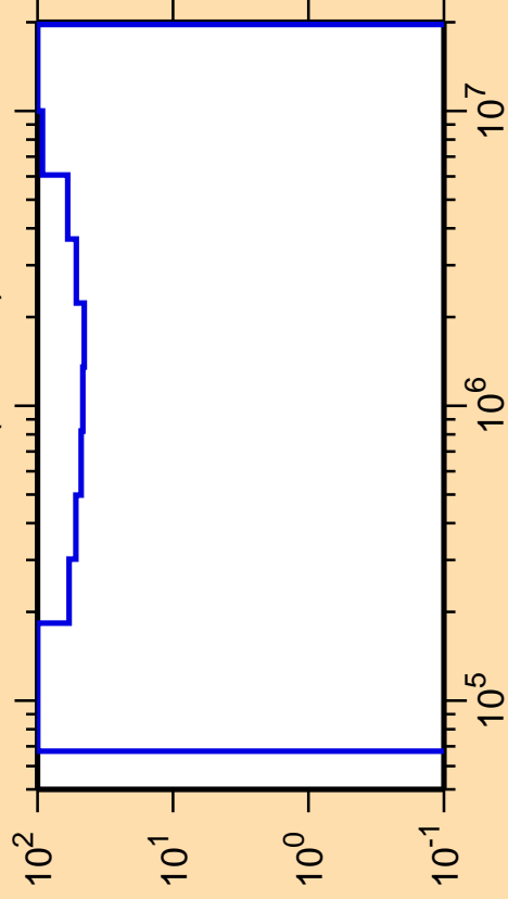
\Delta\sigma/\sigma vs. E for ^{246}\text{Bk}(n,\text{inel.})
