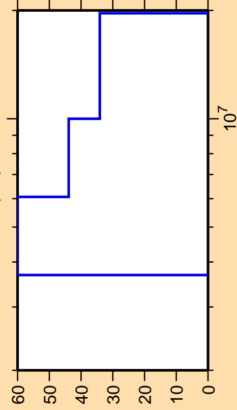
\Delta\sigma/\sigma vs. E for ^{246}\text{Bk}(n,f)
