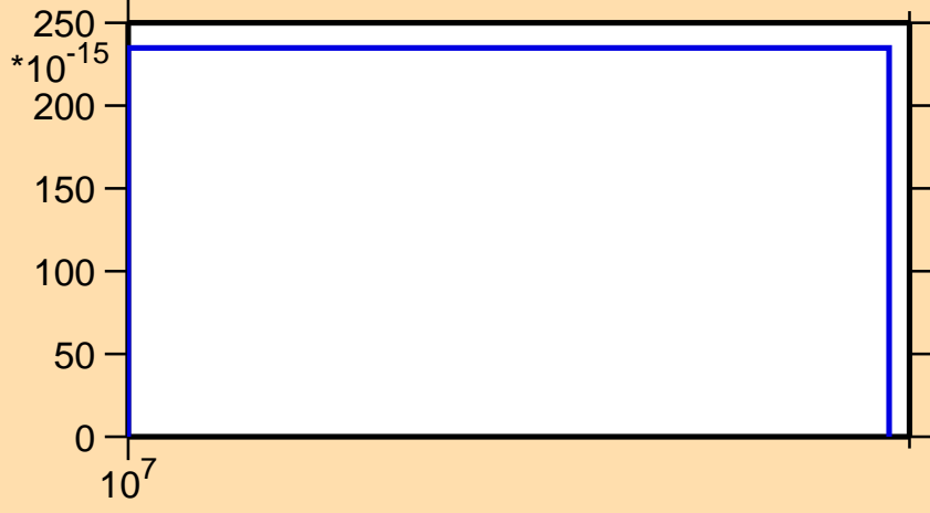
\sigma vs. E for ^{246}\text{Bk}(n,3n\alpha)
