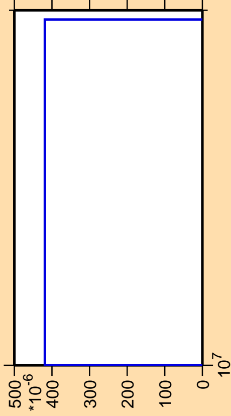
\Delta\sigma/\sigma vs. E for ^{246}\text{Bk} (mt 34)
