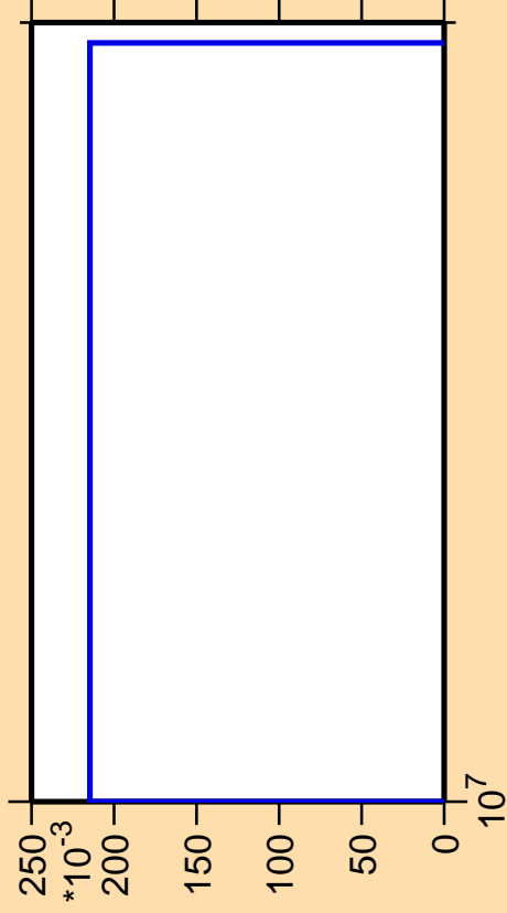
\Delta\sigma/\sigma vs. E for ^{246}\text{Bk}(n,p\alpha)
