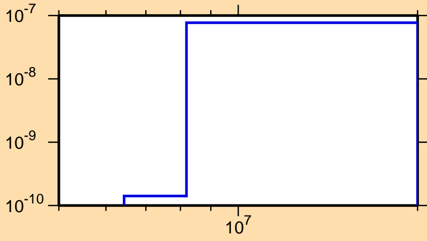
\sigma vs. E for ^{246}\text{Bk}(n,2n\alpha)
