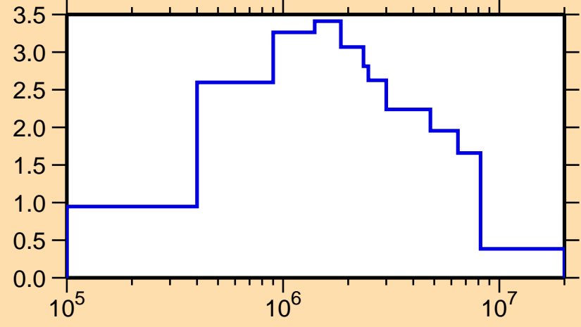
\sigma vs. E for ^{246}\text{Bk}(n,\text{inel.})
