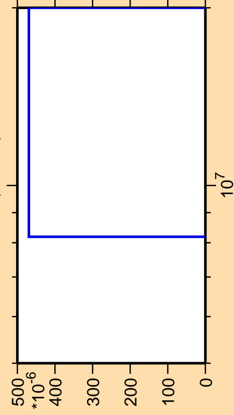
\Delta\sigma/\sigma vs. E for ^{246}\text{Bk}(\text{mt } 34)
