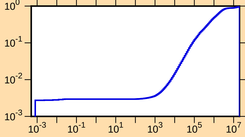
\mu vs. E for ^{247}\text{Bk}(\text{mt251})
