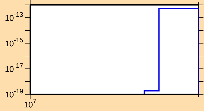
\sigma vs. E for ^{247}\text{Bk}(\text{mt 11})
