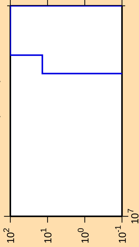
\Delta\sigma/\sigma vs. E for ^{247}\text{Bk}(n,\text{He3})
