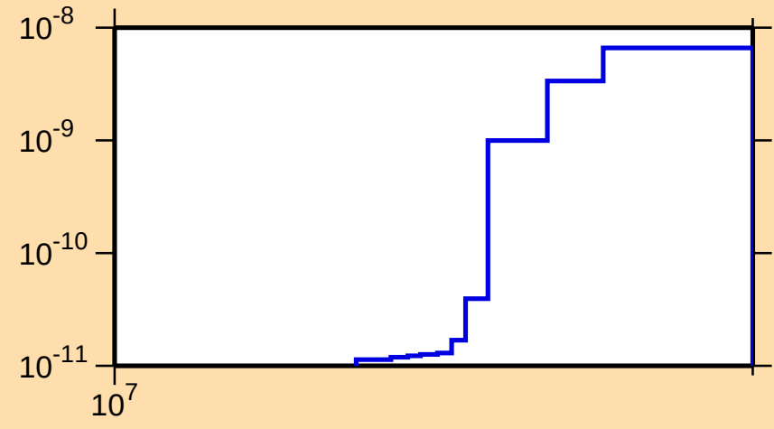
\sigma vs. E for ^{247}\text{Bk}(n,3n\alpha)
