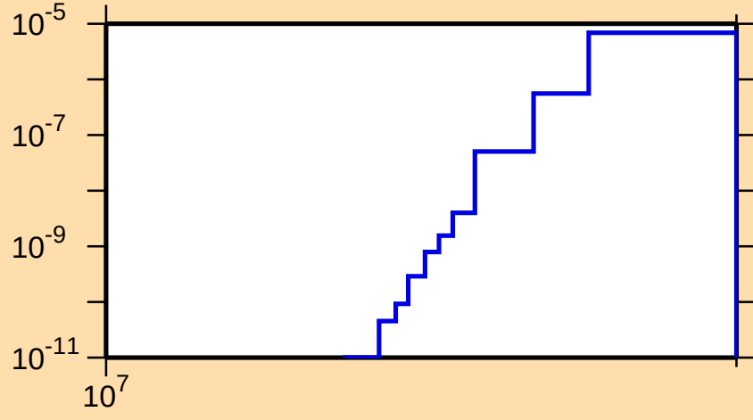
\sigma vs. E for ^{247}\text{Bk}(n,nt)
