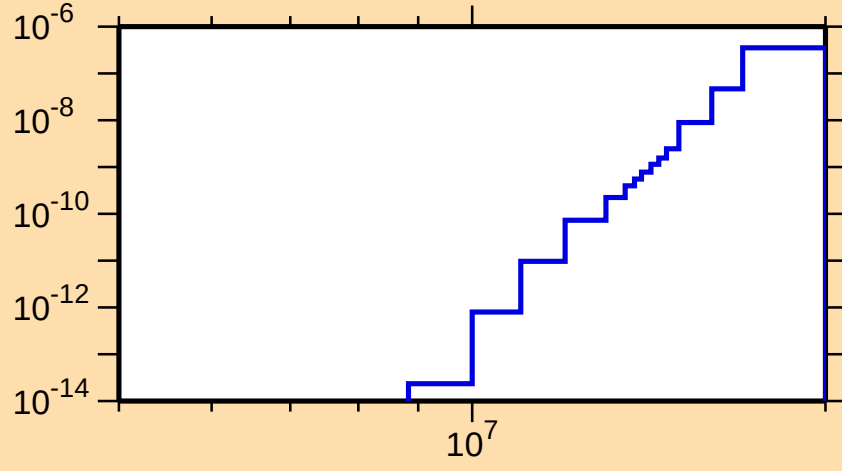
\sigma vs. E for ^{247}\text{Bk}(n,2n\alpha)
