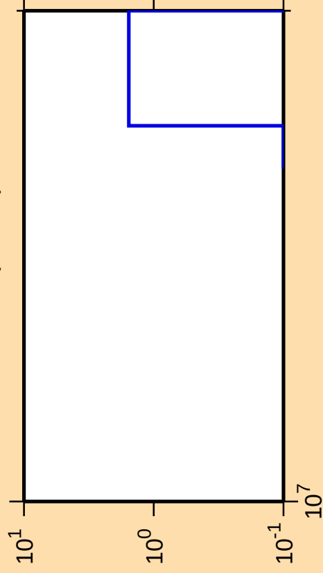
\Delta\sigma/\sigma vs. E for ^{247}\text{Bk}(\text{mt 11})
