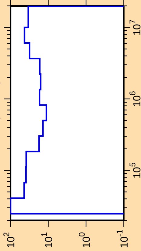
\Delta\sigma/\sigma vs. E for ^{247}\text{Bk}(n,\text{inel.})
