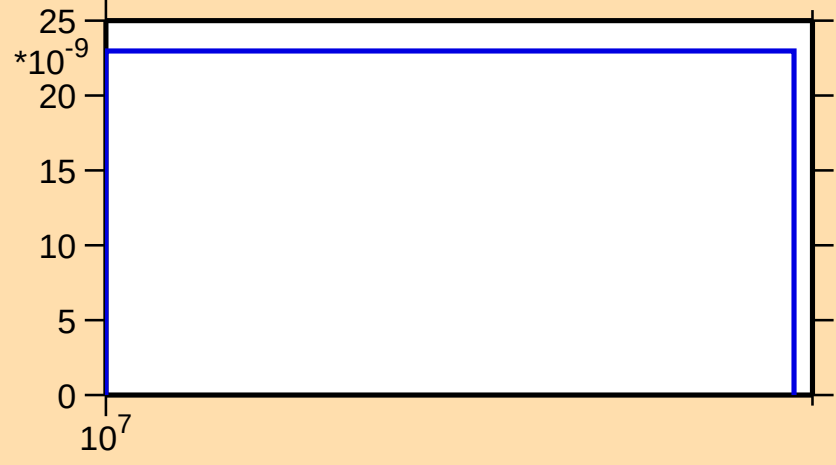
\sigma vs. E for ^{247}\text{Bk}(n,\text{nd})
