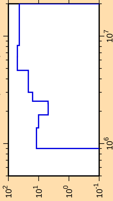
\Delta\sigma/\sigma vs. E for ^{247}\text{Bk}(n,\text{ncont.})
