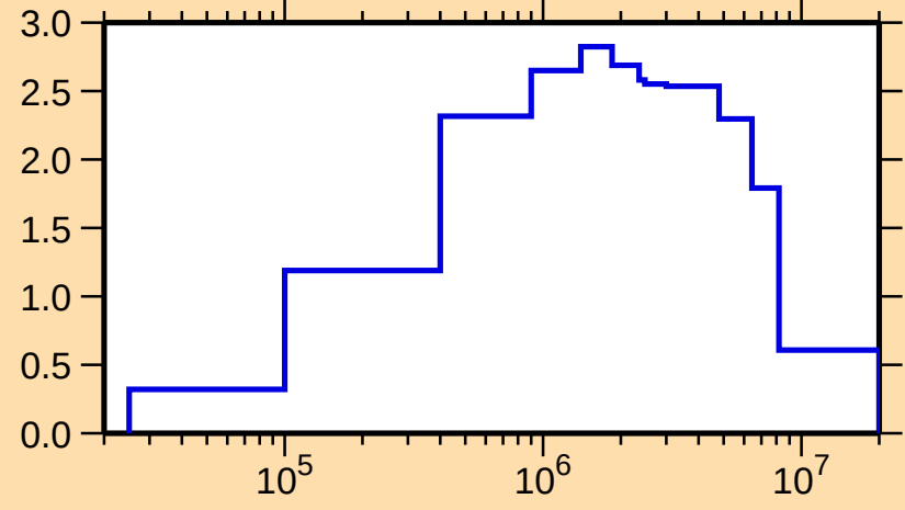
\sigma vs. E for ^{247}\text{Bk}(n,\text{inel.})
