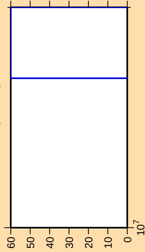
\Delta\sigma/\sigma vs. E for ^{248}\text{Bk}(n,\text{He3})
