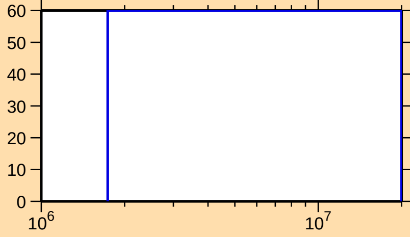
\Delta\sigma/\sigma vs. E for ^{248}\text{Bk}(n,\gamma)
