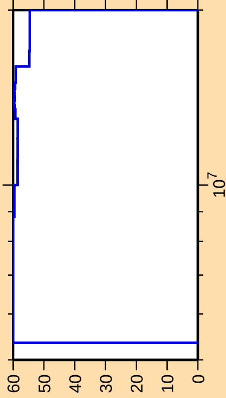
\Delta\sigma/\sigma vs. E for ^{248}\text{Bk}(n,f)
