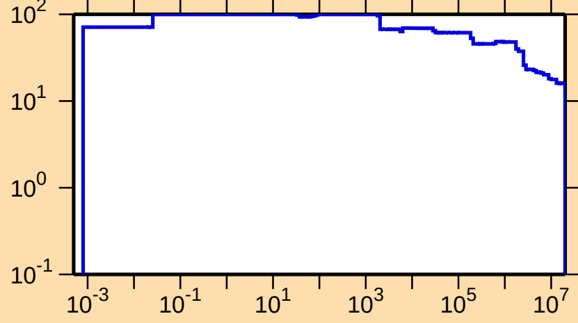
\Delta\sigma/\sigma vs. E for ^{248}\text{Bk}(n,\text{nonel.})
