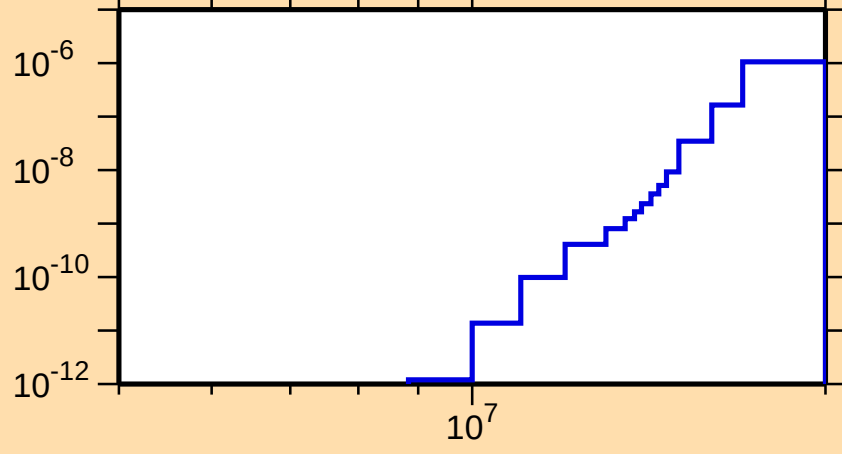
\sigma vs. E for ^{248}\text{Bk}(n,2n\alpha)
