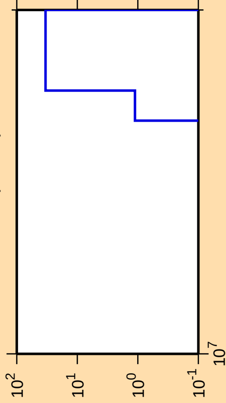
\Delta\sigma/\sigma vs. E for ^{248}\text{Bk}(n,3n\alpha)
