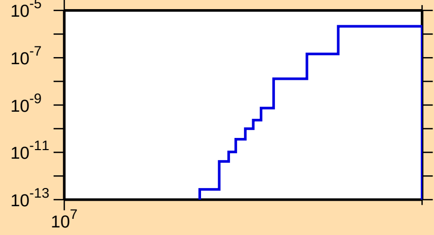
\sigma vs. E for ^{248}\text{Bk}(n,2np)
