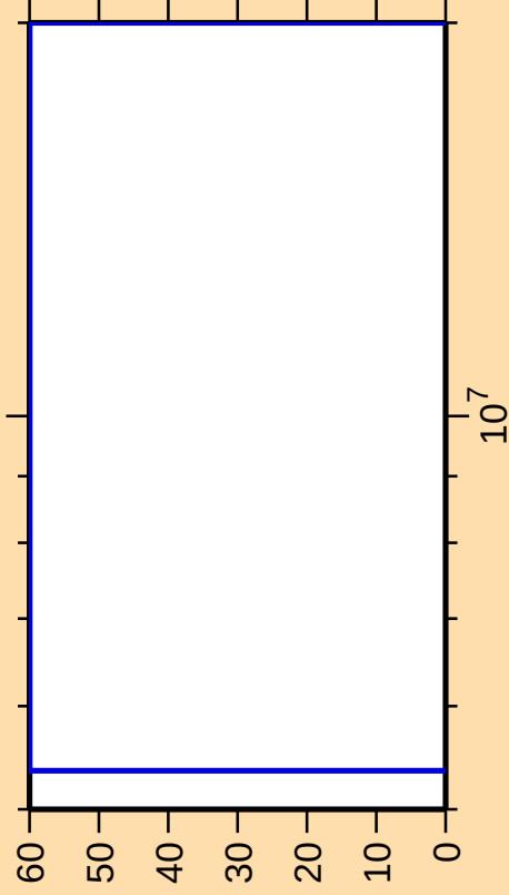
\Delta\sigma/\sigma vs. E for ^{248}\text{Bk}(n,2n)
