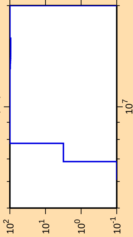
\Delta\sigma/\sigma vs. E for ^{248}\text{Bk}(n,t)
