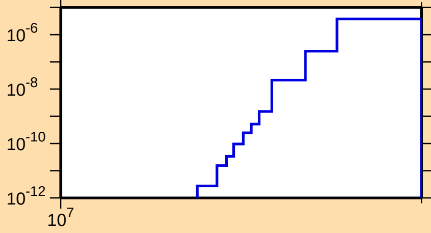
\sigma vs. E for ^{248}\text{Bk}(n,nt)
