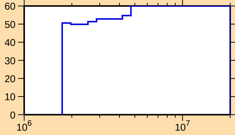
\Delta\sigma/\sigma vs. E for ^{248}\text{Bk}(n,n\text{cont.})
