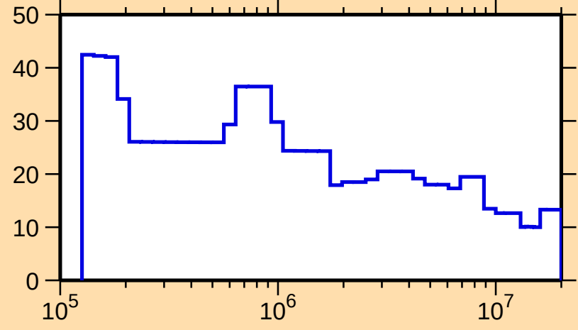
\Delta\sigma/\sigma vs. E for ^{248}\text{Bk}(n,\text{tot.})
