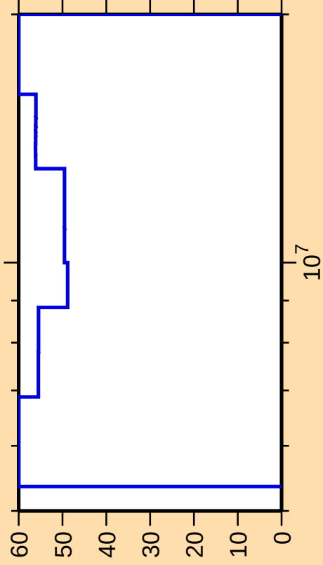
\Delta\sigma/\sigma vs. E for ^{248}\text{Bk}(n,p)
