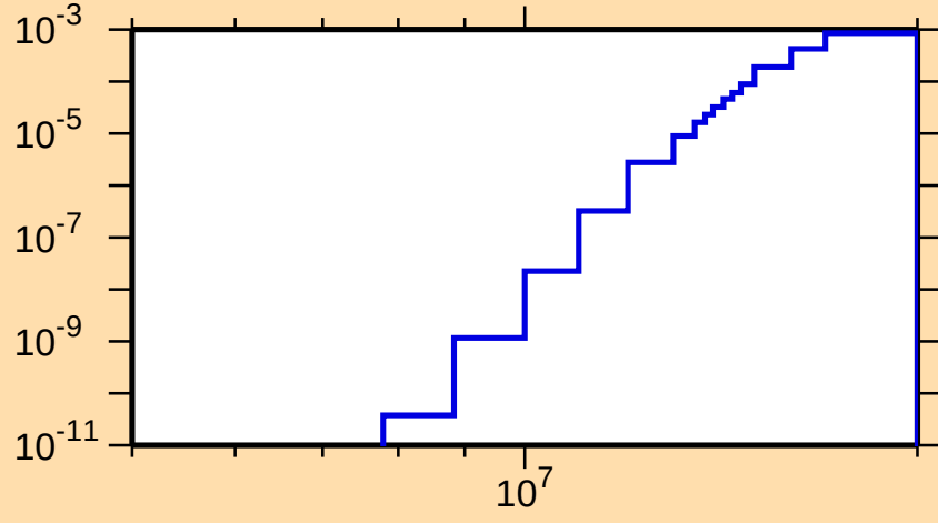
\sigma vs. E for ^{248}\text{Bk}(n,t)
