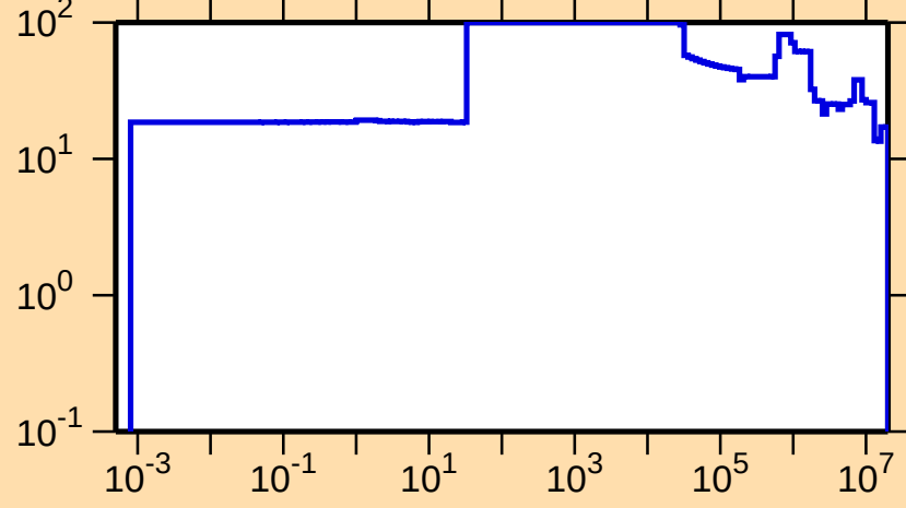
\Delta\sigma/\sigma vs. E for ^{248}\text{Bk}(n,\text{el.})
