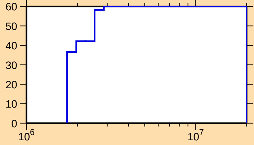
\Delta\sigma/\sigma vs. E for ^{248}\text{Bk}(n,n_1)
