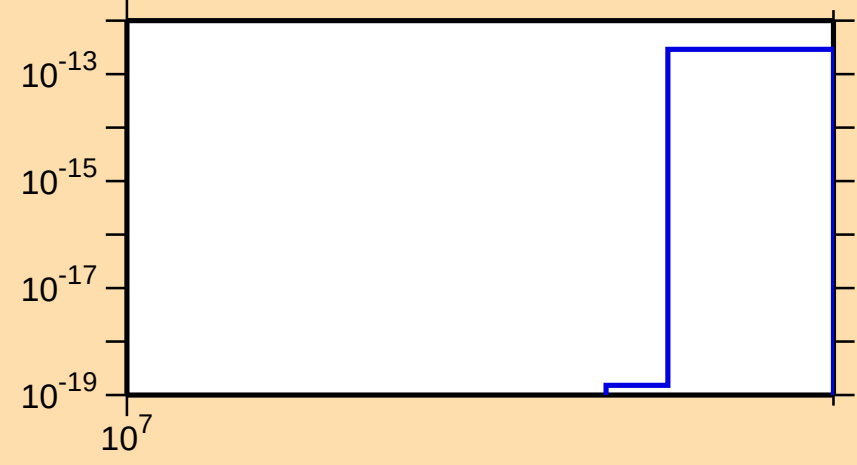
\sigma vs. E for ^{248}\text{Bk}(\text{mt 11})
