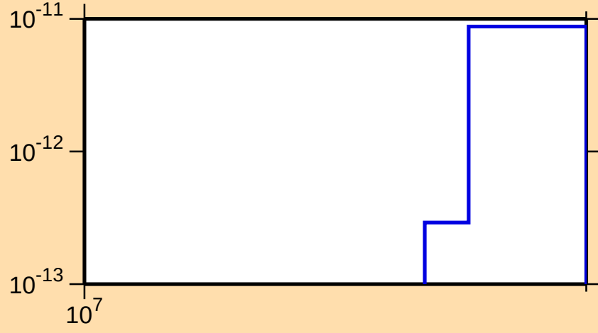
\sigma vs. E for ^{248}\text{Bk}(n,3n\alpha)
