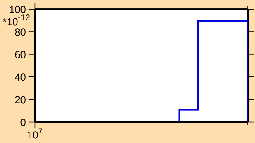
\sigma vs. E for ^{248}\text{Bk}(n,\text{He3})
