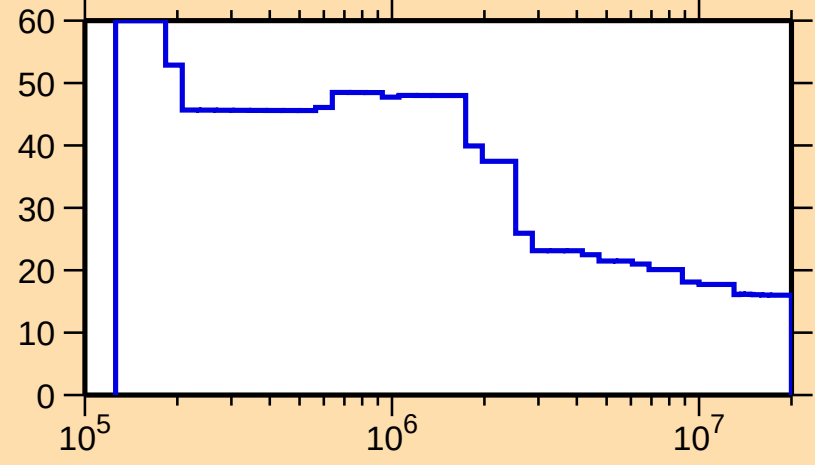
\Delta\sigma/\sigma vs. E for ^{248}\text{Bk}(n,\text{nonel.})
