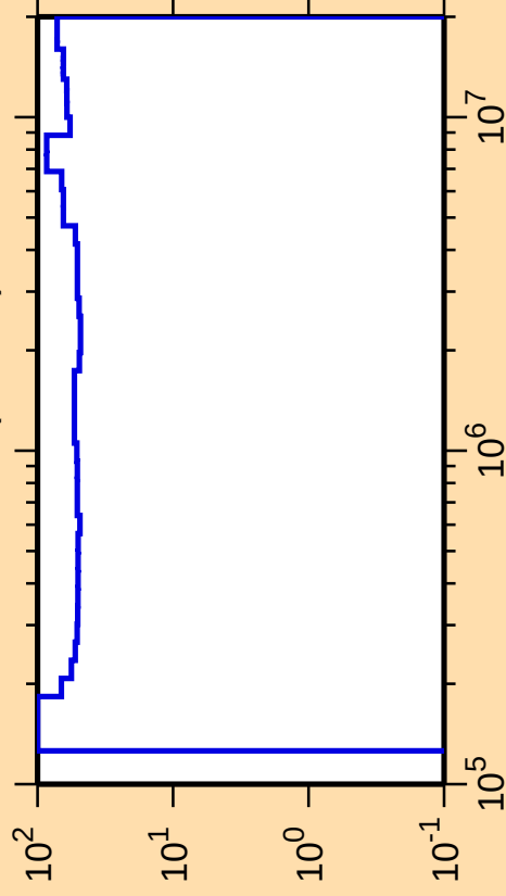
\Delta\sigma/\sigma vs. E for ^{248}\text{Bk}(n,\text{inel.})
