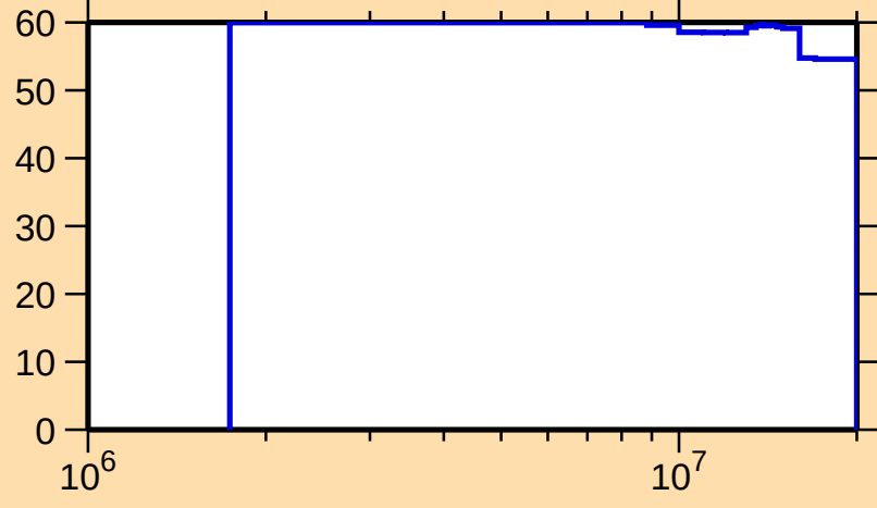
\Delta\sigma/\sigma vs. E for ^{248}\text{Bk}(n,f)
