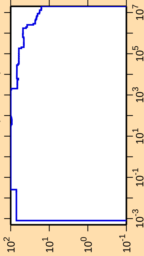
\Delta\sigma/\sigma vs. E for ^{248}\text{Bk}(n,\text{nonel.})
