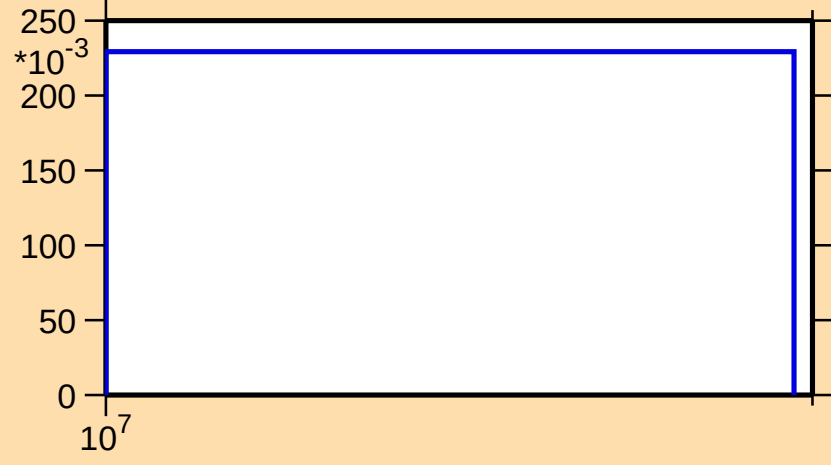
\sigma vs. E for ^{248}\text{Bk}(n,3n)
