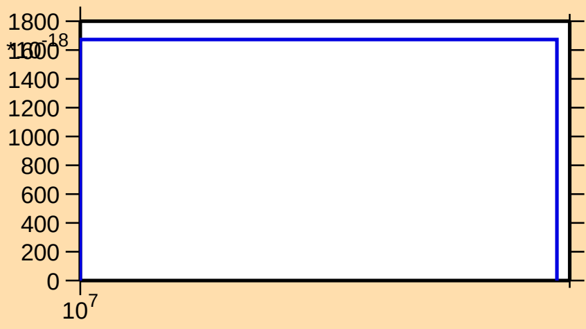
\sigma vs. E for ^{248}\text{Bk}(\text{mt 11})
