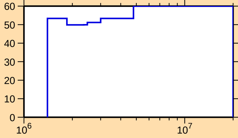
\Delta\sigma/\sigma vs. E for ^{248}\text{Bk}(n,ncont.)
