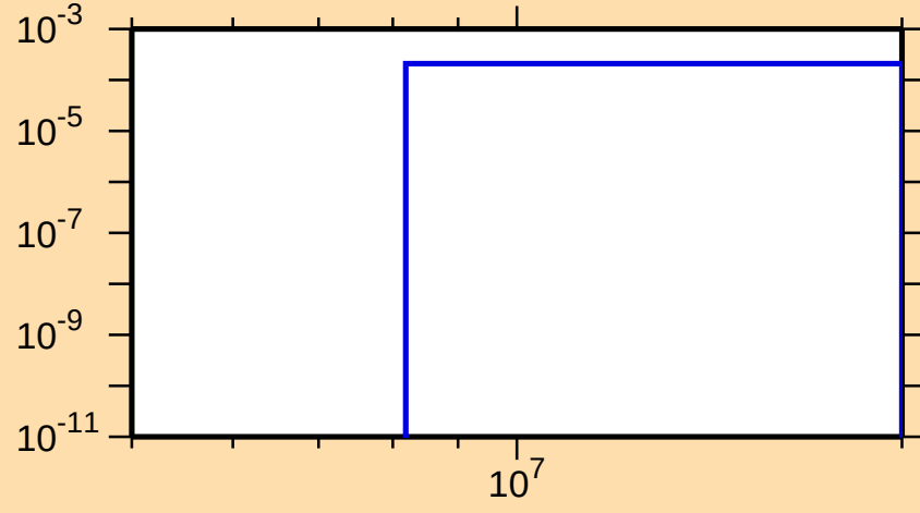
\sigma vs. E for ^{248}\text{Bk}(n,d)
