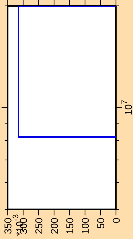
\Delta\sigma/\sigma vs. E for ^{248}\text{Bk}(n,3n\alpha)
