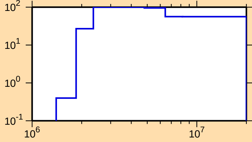
\Delta\sigma/\sigma vs. E for ^{248}\text{Bk}(n,p)
