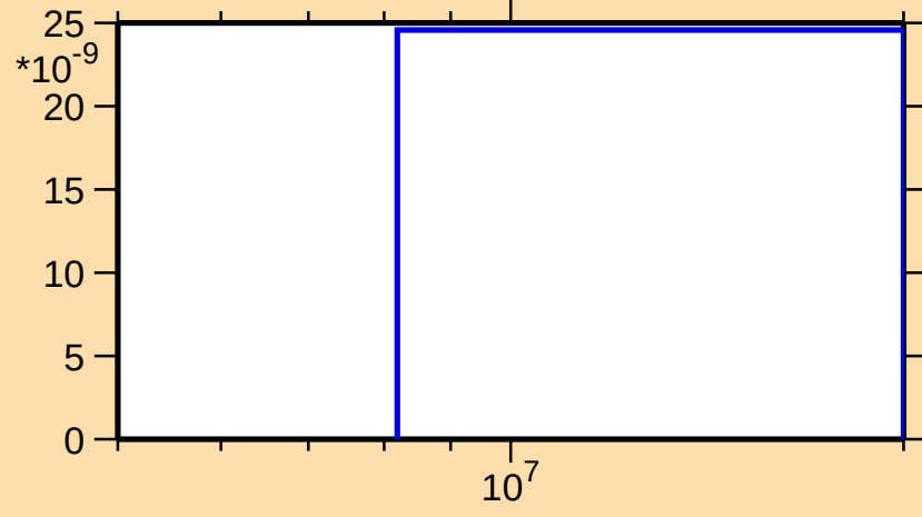
\sigma vs. E for ^{248}\text{Bk}(n,2np)
