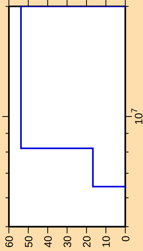
\Delta\sigma/\sigma vs. E for ^{248}\text{Bk}(n,d)
