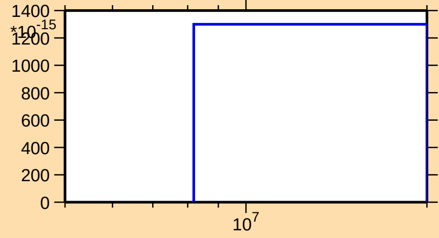
\sigma vs. E for ^{248}\text{Bk}(n,\text{He3})
