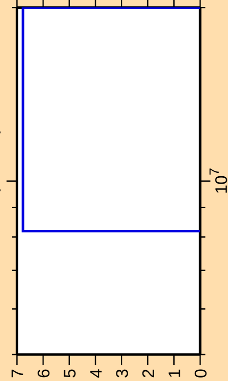
\Delta\sigma/\sigma vs. E for ^{248}\text{Bk}(n,\text{He3})
