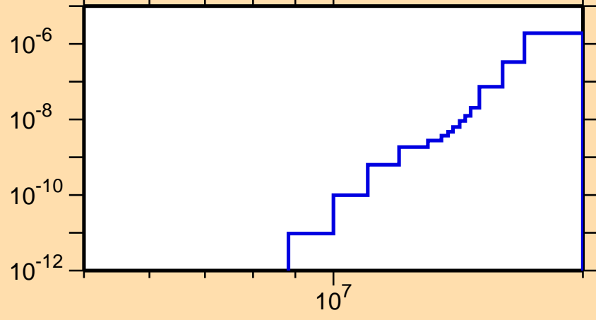
\sigma vs. E for ^{248}\text{Bk}(n,2n\alpha)
