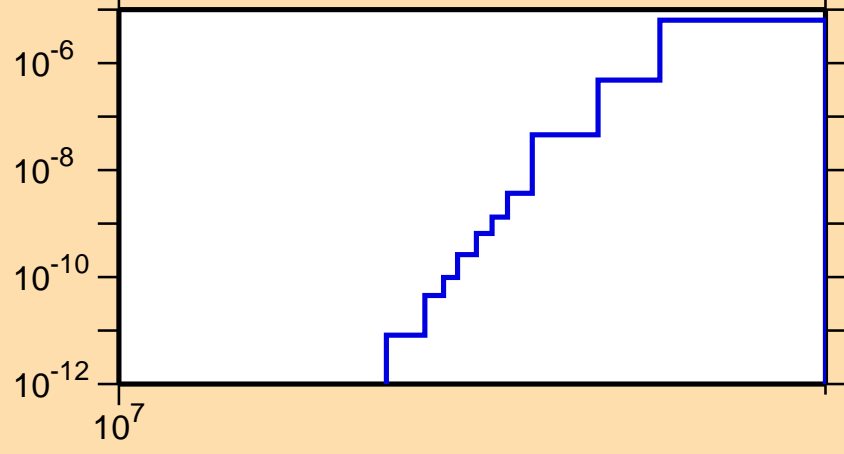
\sigma vs. E for ^{248}\text{Bk}(n,nt)
