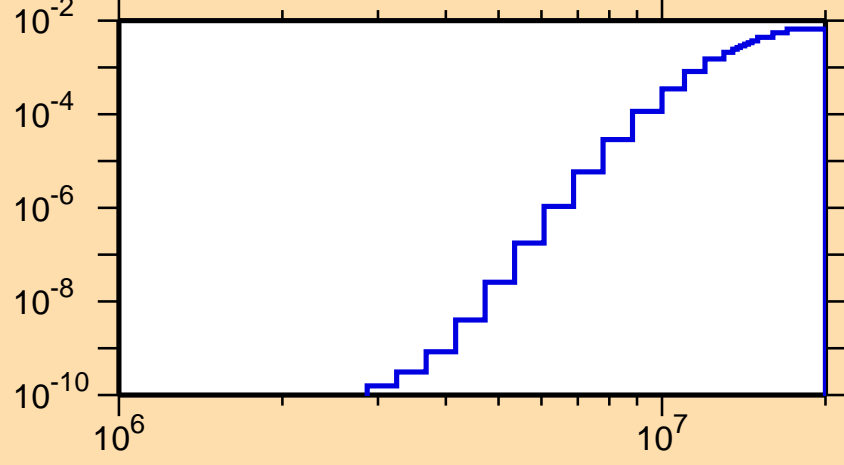
\sigma vs. E for ^{248}\text{Bk}(n,p)
