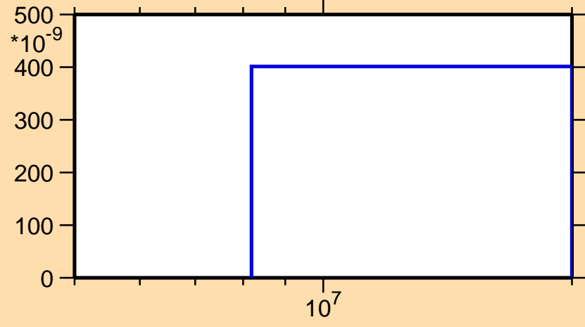
\sigma vs. E for ^{248}\text{Bk}(n,\text{nd})
