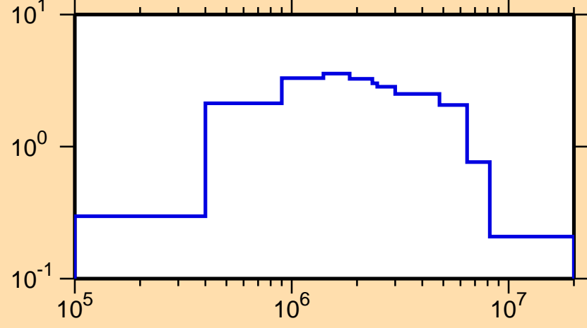
\sigma vs. E for ^{248}\text{Bk}(n,n\text{cont.})
