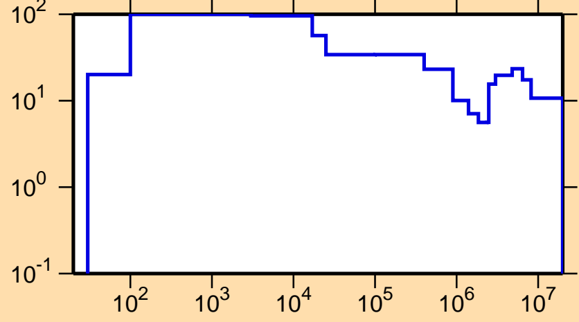
\Delta\sigma/\sigma vs. E for ^{248}\text{Bk}(n,\text{tot.})
