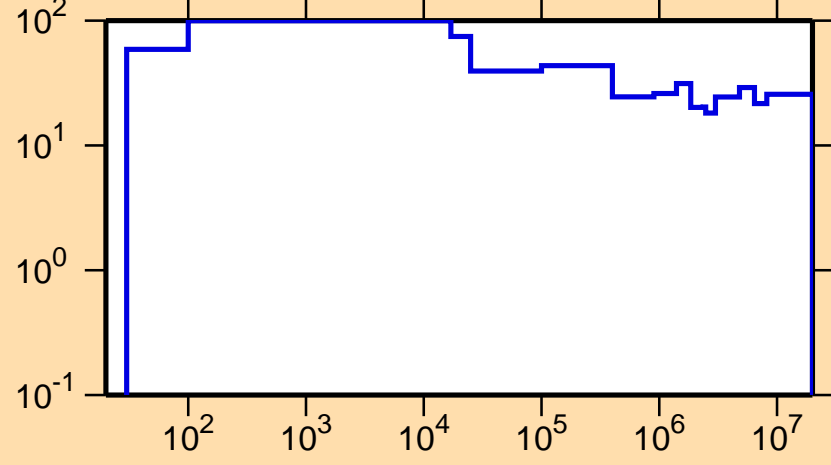
\Delta\sigma/\sigma vs. E for ^{248}\text{Bk}(n,\text{el.})
