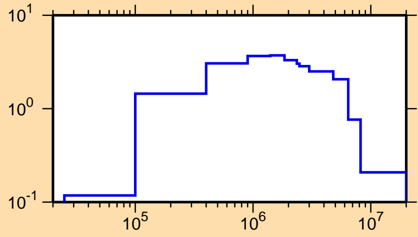
\sigma vs. E for ^{248}\text{Bk}(n,\text{inel.})
