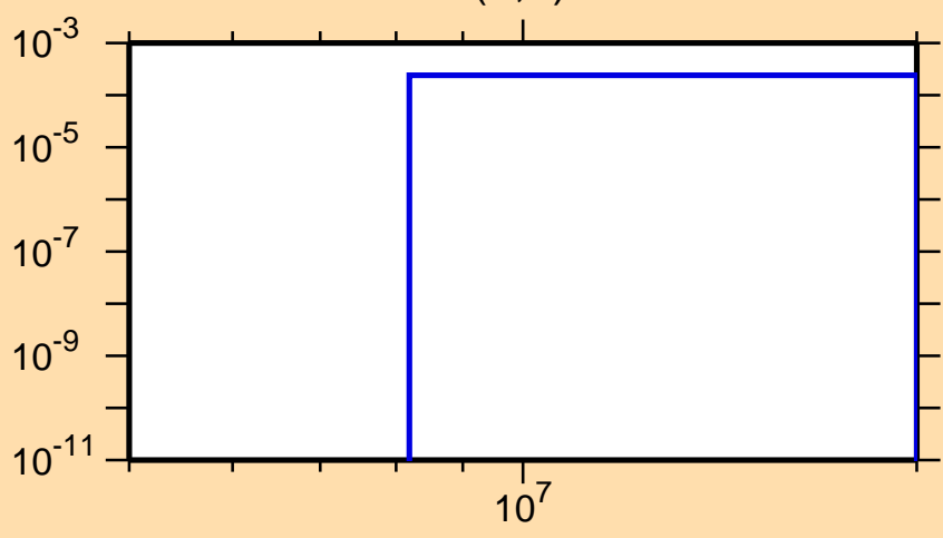
\sigma vs. E for ^{248}\text{Bk}(n,d)
