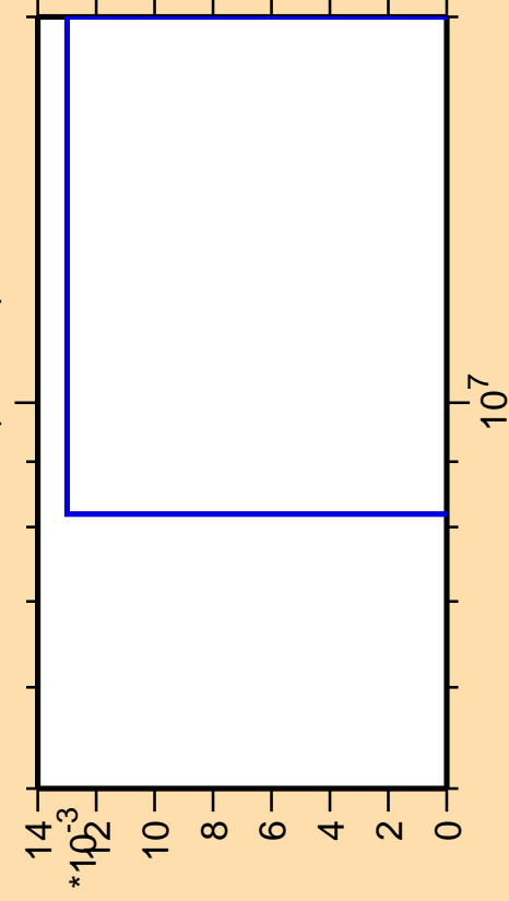
\Delta\sigma/\sigma vs. E for ^{248}\text{Bk} (mt 11)
