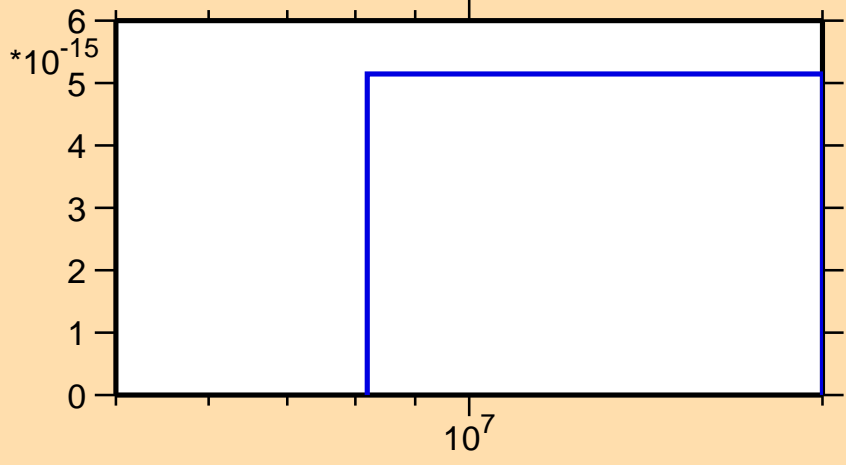
\sigma vs. E for ^{248}\text{Bk} (mt 11)
