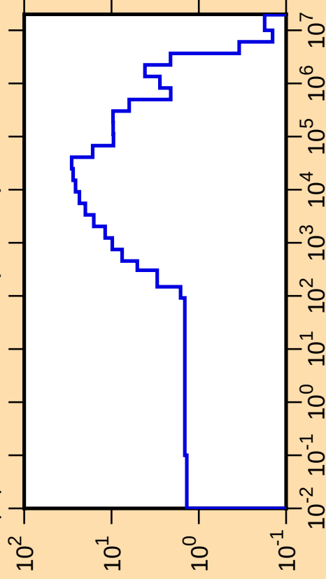
\Delta\mu/\mu vs. E for ^{249}\text{Bk}(\text{mt251})
