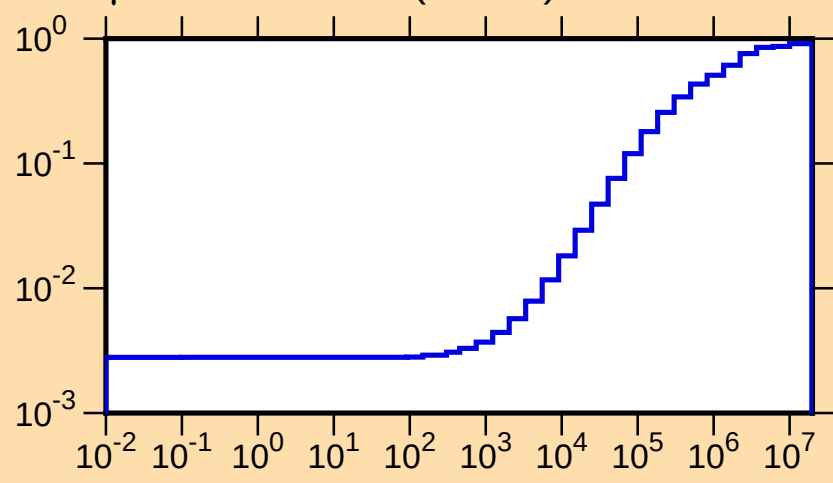
\mu vs. E for ^{249}\text{Bk}(\text{mt251})
