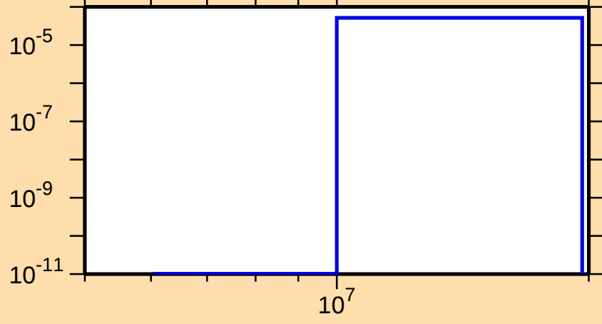
\sigma vs. E for ^{249}\text{Bk}(n,t)
