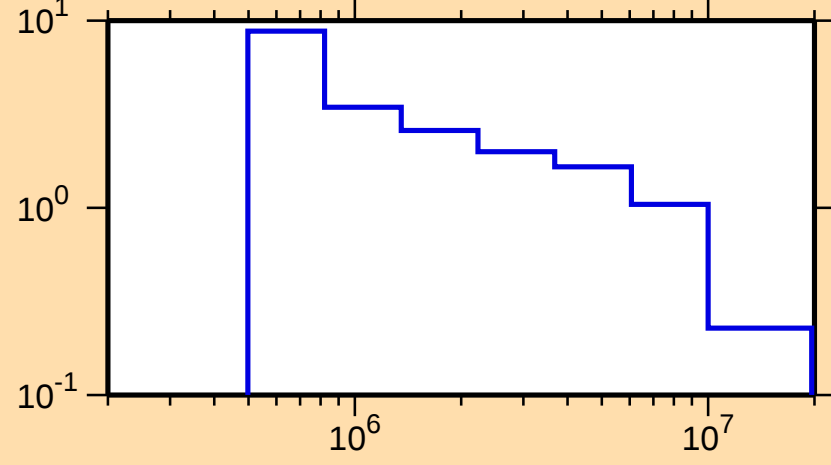
\Delta\sigma/\sigma vs. E for ^{249}\text{Bk}(n,n\text{onel.})
