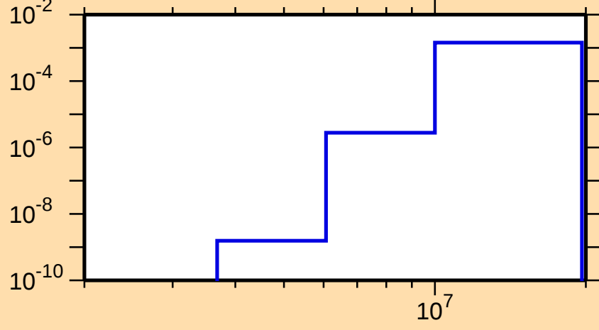
\sigma vs. E for ^{249}\text{Bk}(n,p)
