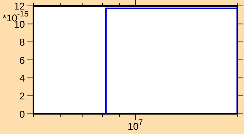
\sigma vs. E for ^{249}\text{Bk}(\text{mt 11})
