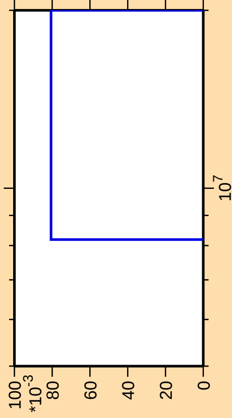
\Delta\sigma/\sigma vs. E for ^{249}\text{Bk}(n,3n\alpha)
