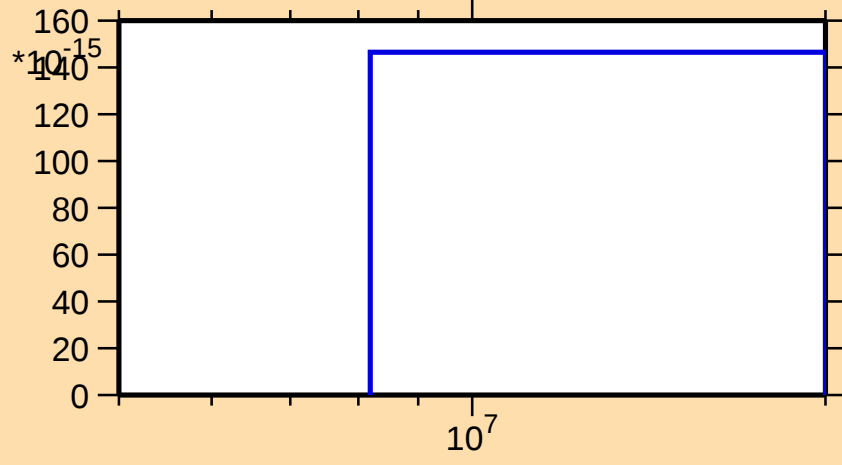
\sigma vs. E for ^{249}\text{Bk}(n,3n\alpha)
