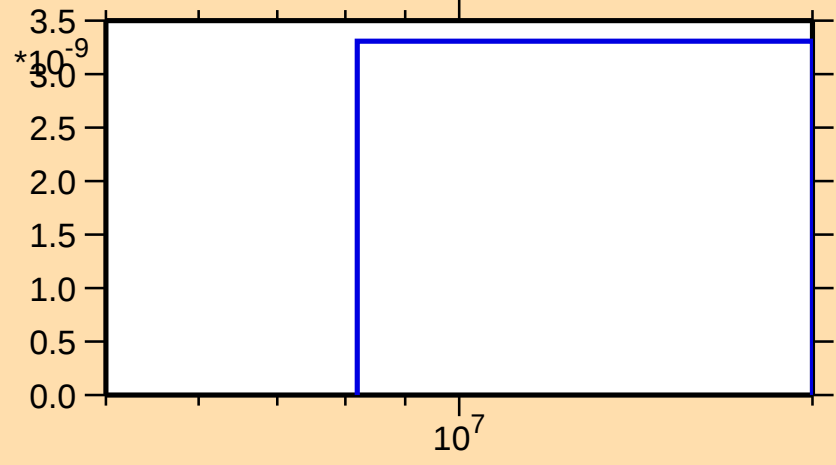
\sigma vs. E for ^{249}\text{Bk}(n,2np)
