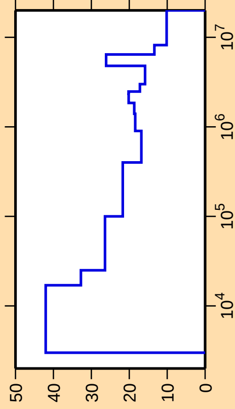
\Delta\sigma/\sigma vs. E for ^{249}\text{Bk}(n,\text{inel.})
