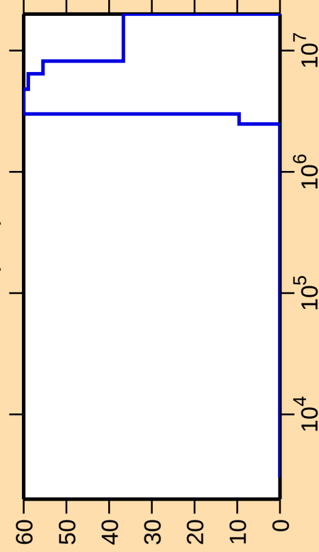
\Delta\sigma/\sigma vs. E for ^{249}\text{Bk}(n,\alpha)
