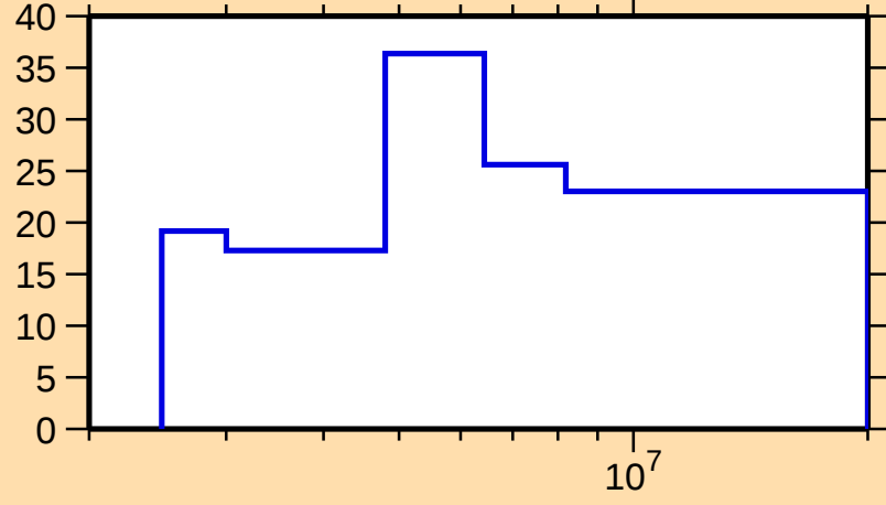
\Delta\sigma/\sigma vs. E for ^{249}\text{Bk}(n,n\text{cont.})
