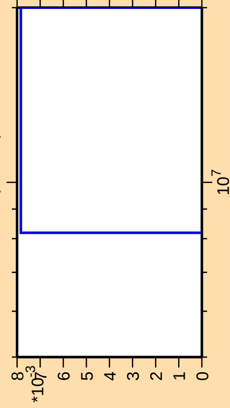
\Delta\sigma/\sigma vs. E for ^{249}\text{Bk}(\text{mt 11})
