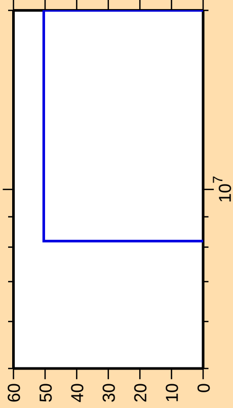
\Delta\sigma/\sigma vs. E for ^{249}\text{Bk}(n,2n\alpha)
