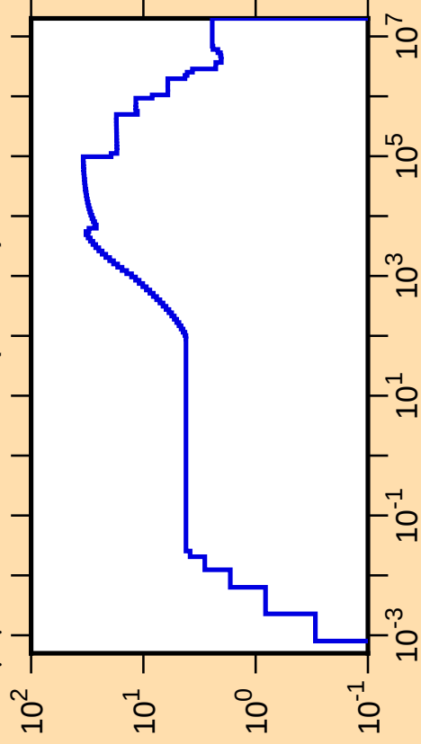
\Delta\mu/\mu vs. E for ^{250}\text{Bk}(\text{mt251})
