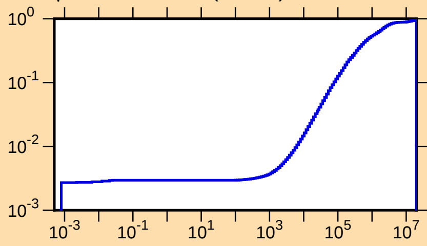
\mu vs. E for ^{250}\text{Bk}(\text{mt251})
