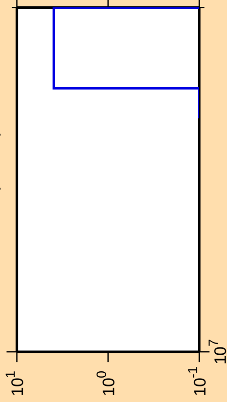
\Delta\sigma/\sigma vs. E for ^{250}\text{Bk}(\text{mt 11})
