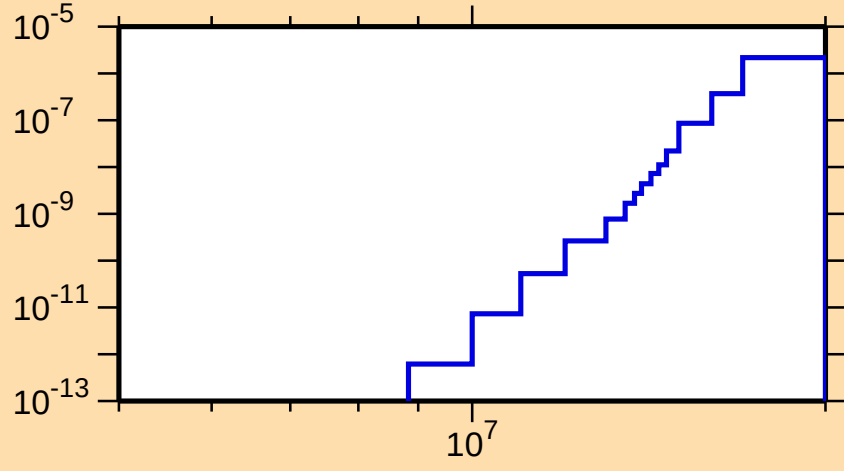
\sigma vs. E for ^{250}\text{Bk}(n,2n\alpha)
