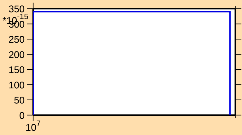
\sigma vs. E for ^{250}\text{Bk}(n,\text{He}3)
