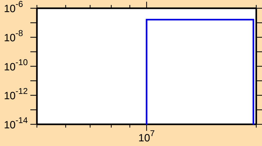
\sigma vs. E for ^{250}\text{Bk}(n,nt)
