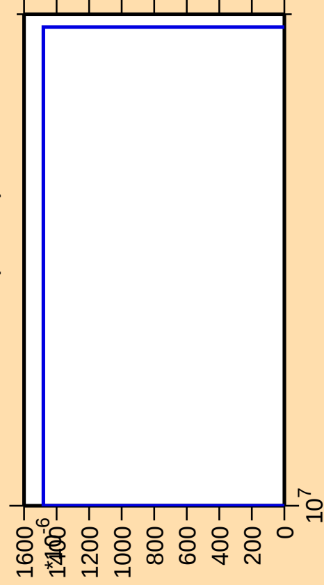
\Delta\sigma/\sigma vs. E for ^{250}\text{Bk}(\text{mt } 42)
