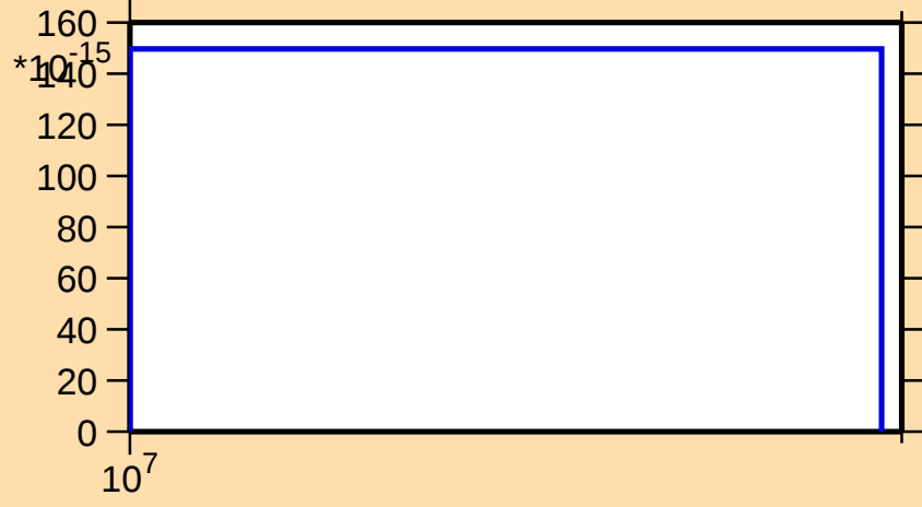
\sigma vs. E for ^{250}\text{Bk}(n,3n\alpha)
