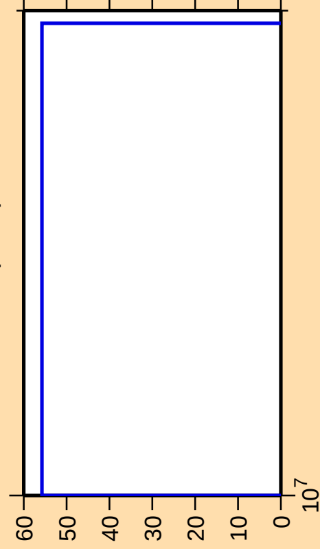
\Delta\sigma/\sigma vs. E for ^{250}\text{Bk}(n,\text{nd})
