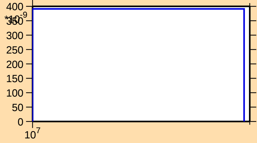
\sigma vs. E for ^{250}\text{Bk}(n,\text{nd})
