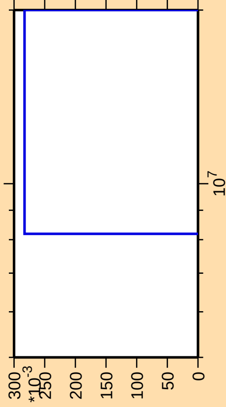
\Delta\sigma/\sigma vs. E for ^{250}\text{Bk}(n,3n\alpha)
