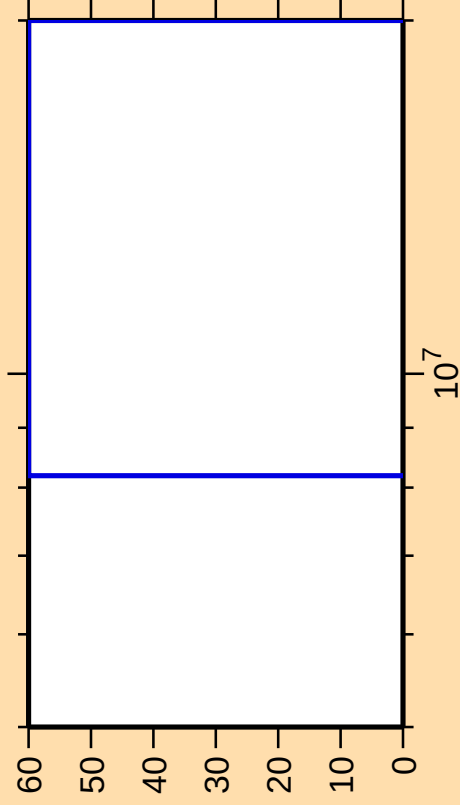
\Delta\sigma/\sigma vs. E for ^{250}\text{Bk}(n,2n\alpha)
