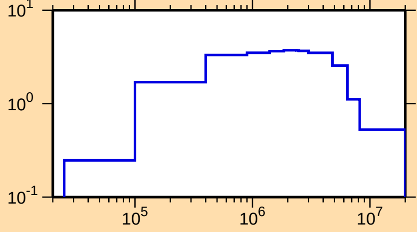
\sigma vs. E for ^{250}\text{Bk}(n,\text{inel.})
