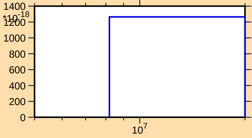
\sigma vs. E for ^{250}\text{Bk}(\text{mt } 42)
