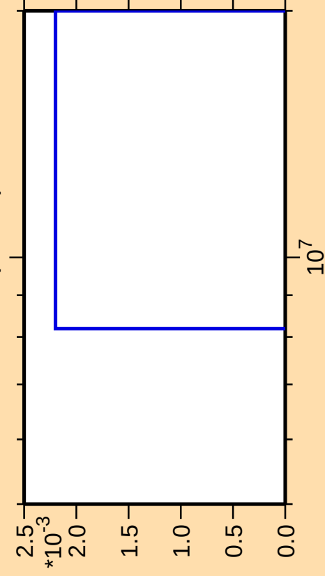
\Delta\sigma/\sigma vs. E for ^{250}\text{Bk}(\text{mt } 42)
