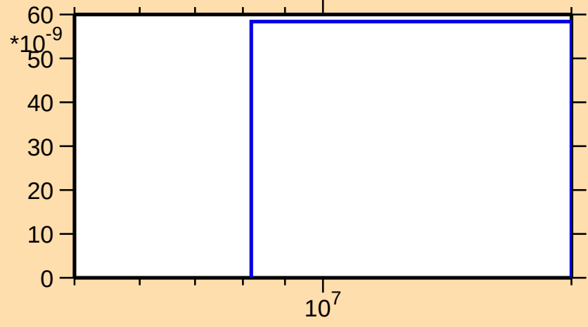
\sigma vs. E for ^{250}\text{Bk}(n,2np)
