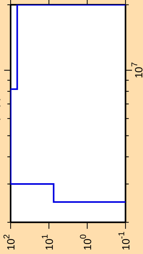
\Delta\sigma/\sigma vs. E for ^{250}\text{Bk}(n,p)
