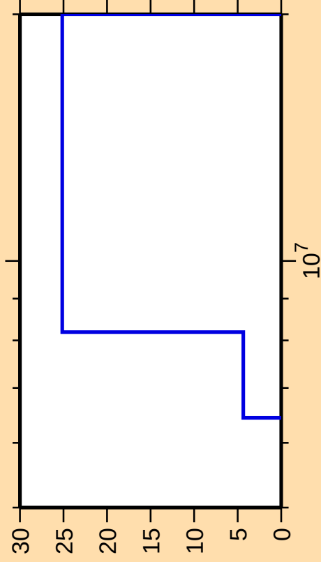
\Delta\sigma/\sigma vs. E for ^{250}\text{Bk}(n,t)
