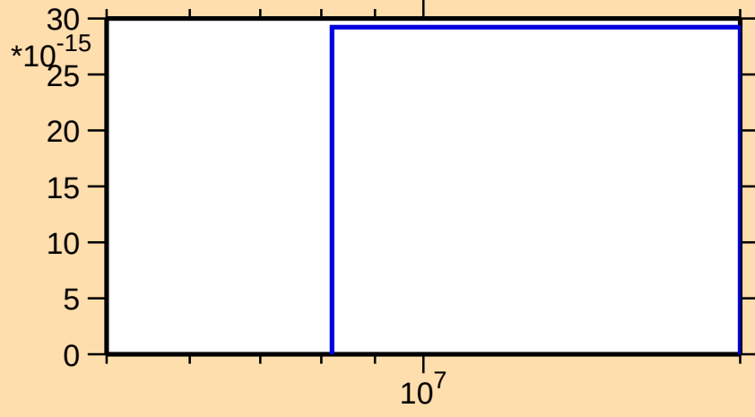
\sigma vs. E for ^{250}\text{Bk}(\text{mt 11})
