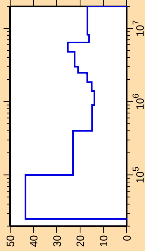
\Delta\sigma/\sigma vs. E for ^{250}\text{Bk}(n,\text{inel.})
