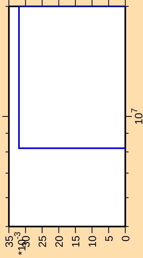
\Delta\sigma/\sigma vs. E for ^{250}\text{Bk}(\text{mt 11})
