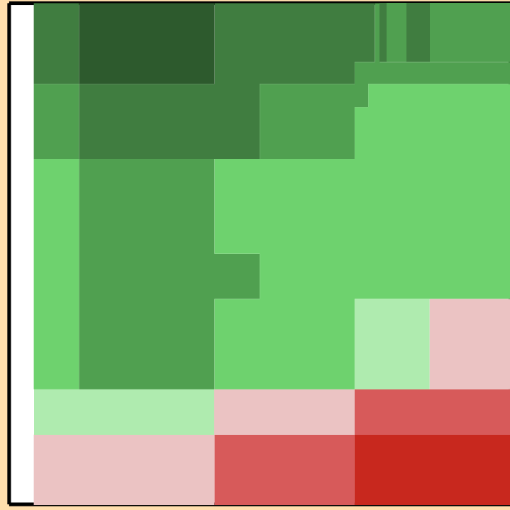
\Delta\sigma/\sigma vs. E for ^{251}\text{Bk}(n,2n)
