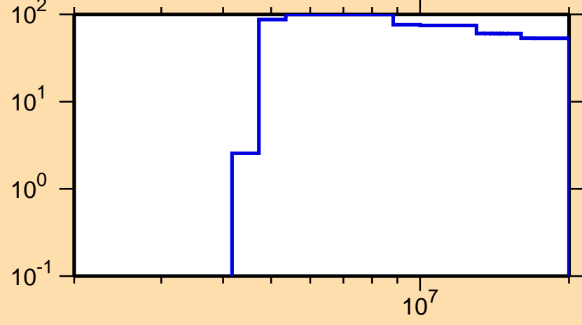
\Delta\sigma/\sigma vs. E for ^{251}\text{Bk}(n,p)
