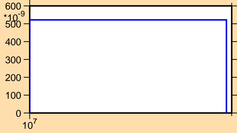
\sigma vs. E for ^{251}\text{Bk}(n,nt)
