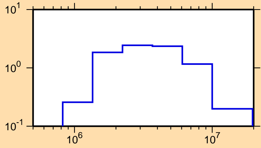
\sigma vs. E for ^{251}\text{Bk}(n,n\text{cont.})
