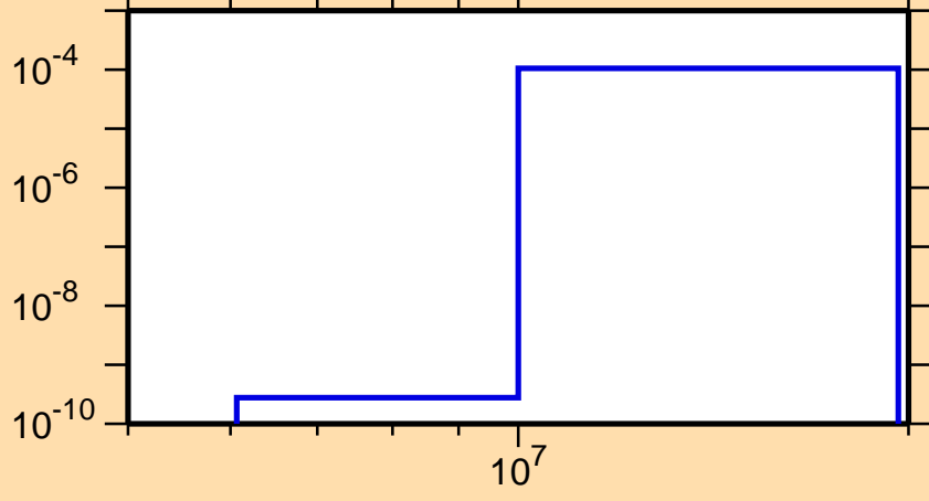
\sigma vs. E for ^{251}\text{Bk}(n,d)
