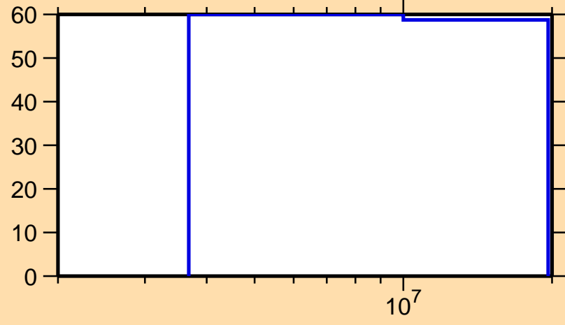
\Delta\sigma/\sigma vs. E for ^{251}\text{Bk}(n,p)
