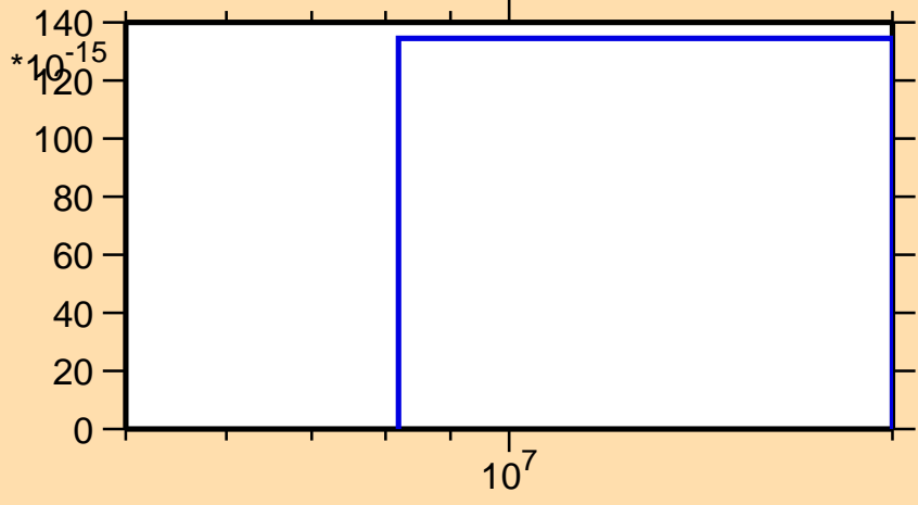
\sigma vs. E for ^{251}\text{Bk} (mt 11)
