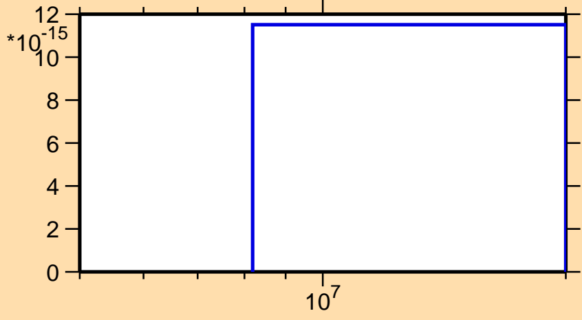
\sigma vs. E for ^{251}\text{Bk} (mt 42)
