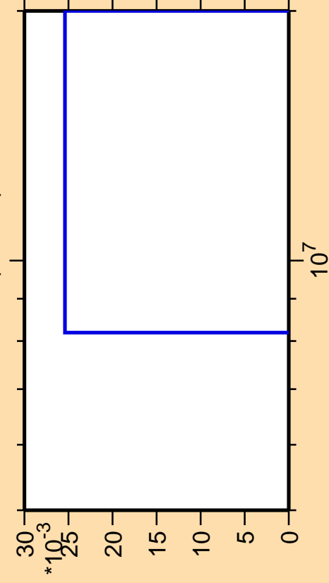
\Delta\sigma/\sigma vs. E for ^{251}\text{Bk} (mt 42)
