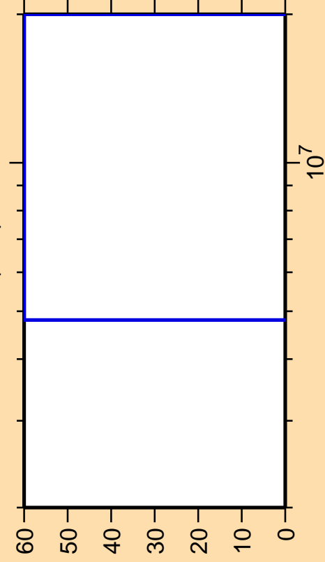
\Delta\sigma/\sigma vs. E for ^{251}\text{Bk}(n,\alpha)
