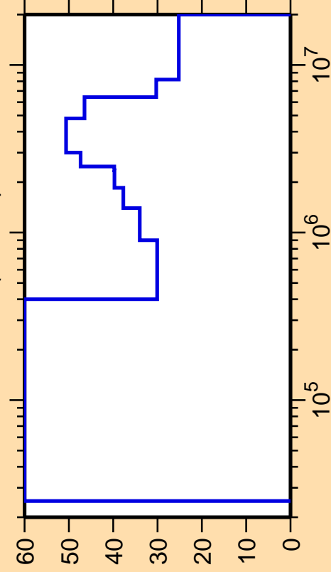
\Delta\sigma/\sigma vs. E for ^{251}\text{Bk}(n,\text{inel.})
