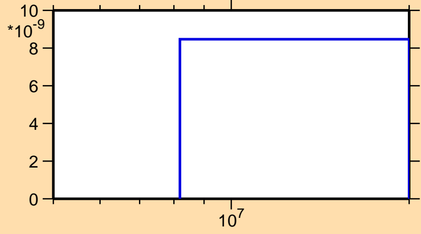
\sigma vs. E for ^{251}\text{Bk}(n,2np)
