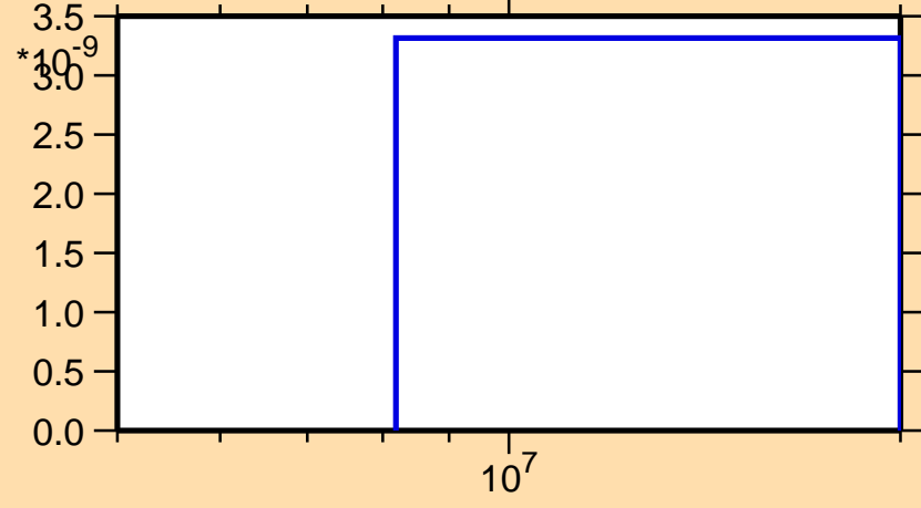
\sigma vs. E for ^{251}\text{Bk}(n,2n\alpha)
