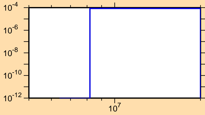
\sigma vs. E for ^{251}\text{Bk}(n,d)
