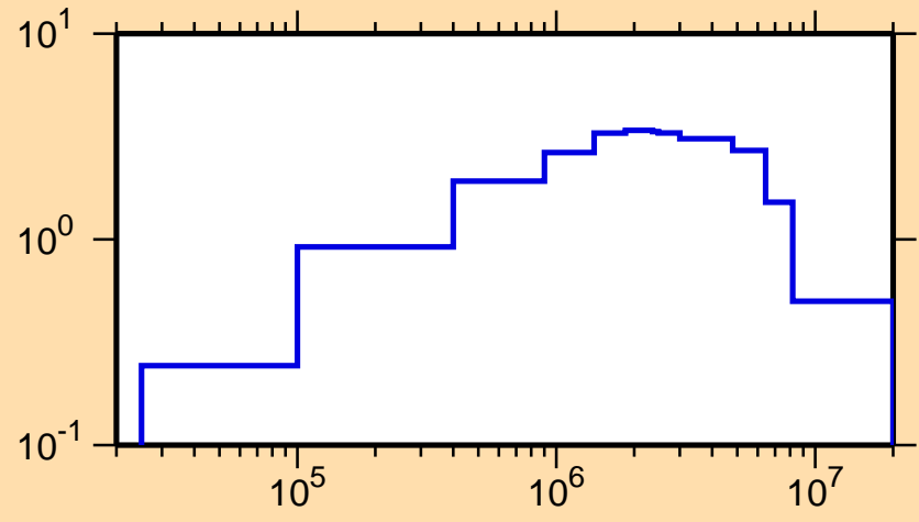
\sigma vs. E for ^{251}\text{Bk}(n,\text{inel.})
