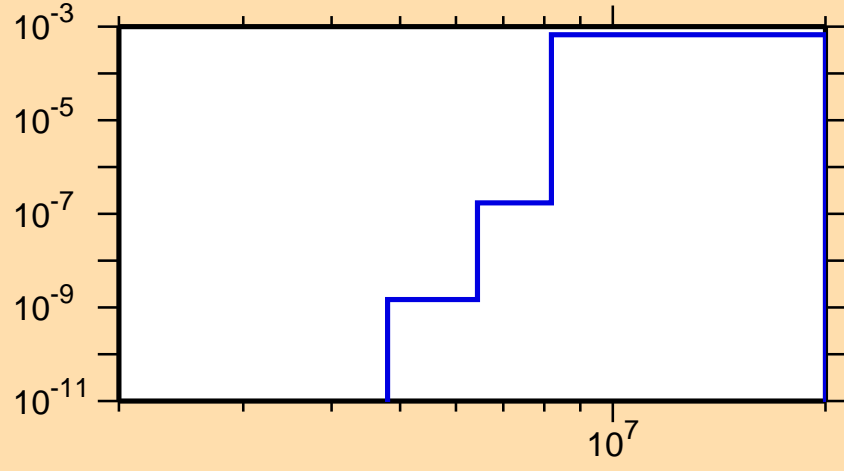
\sigma vs. E for ^{251}\text{Bk}(n,p)
