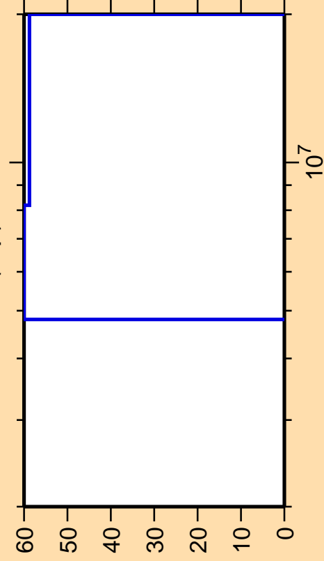
\Delta\sigma/\sigma vs. E for ^{251}\text{Bk}(n,p)
