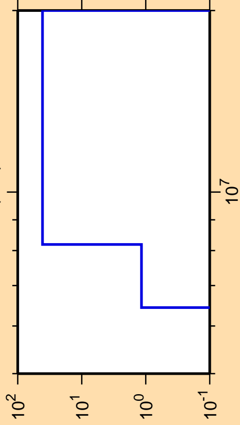
\Delta\sigma/\sigma vs. E for ^{251}\text{Bk}(n,d)
