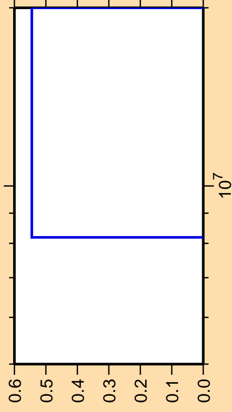
\Delta\sigma/\sigma vs. E for ^{251}\text{Bk} (mt 11)
