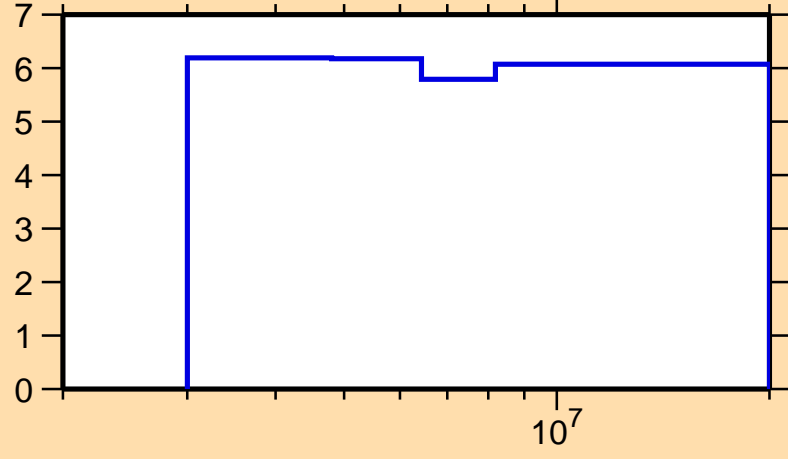
\Delta\sigma/\sigma vs. E for ^{251}\text{Bk}(n,\text{nonel.})
