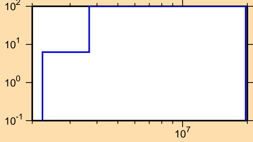
\Delta\sigma/\sigma vs. E for ^{252}\text{Bk}(n,p)
