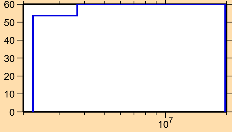
\Delta\sigma/\sigma vs. E for ^{252}\text{Bk}(n,ncont.)
