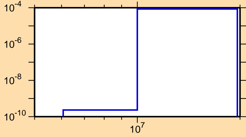
\sigma vs. E for ^{252}\text{Bk}(n,t)
