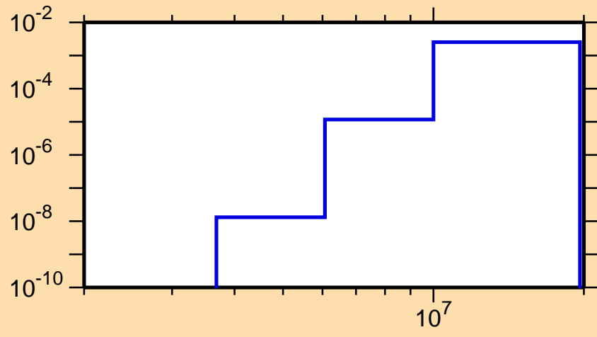
\sigma vs. E for ^{252}\text{Bk}(n,p)
