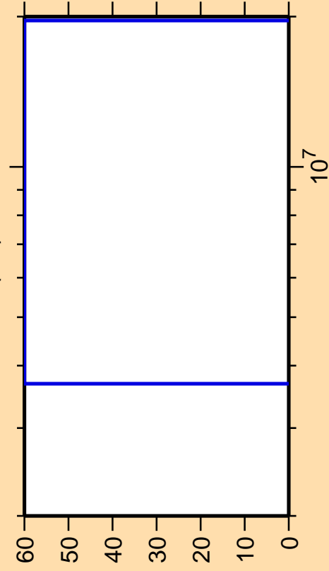
\Delta\sigma/\sigma vs. E for ^{252}\text{Bk}(n,f)
