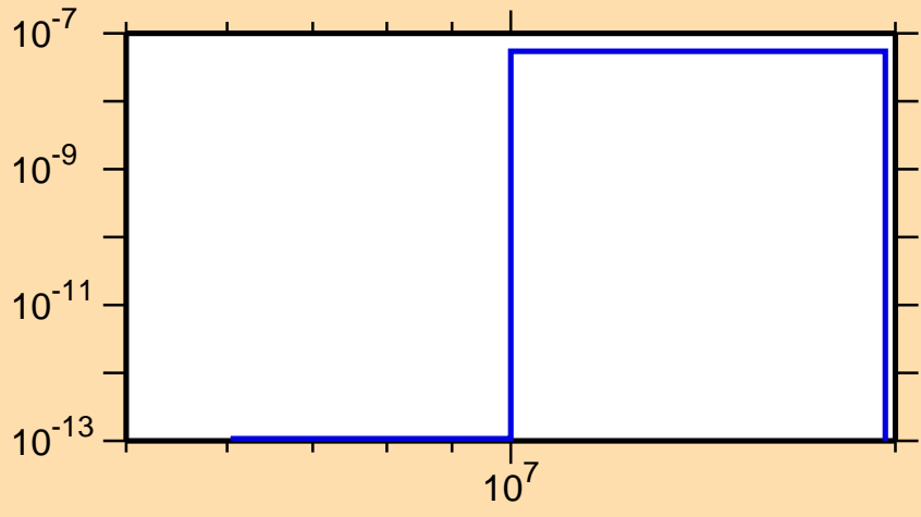
\sigma vs. E for ^{252}\text{Bk}(n,2n\alpha)
