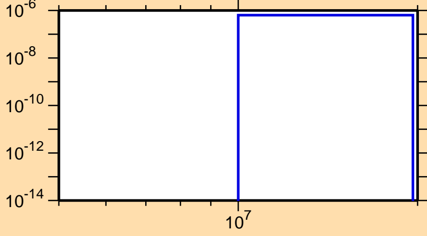
\sigma vs. E for ^{252}\text{Bk}(n,nt)
