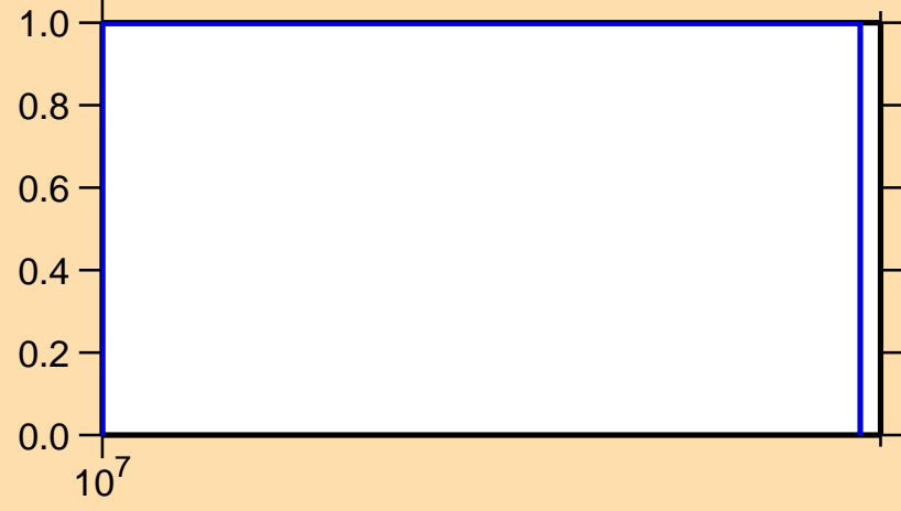
\sigma vs. E for ^{252}\text{Bk}(n,3n)
