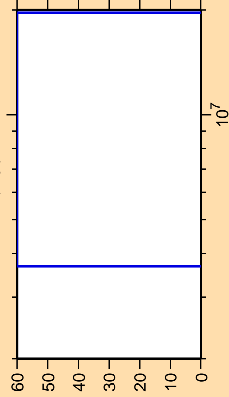
\Delta\sigma/\sigma vs. E for ^{252}\text{Bk}(n,p)
