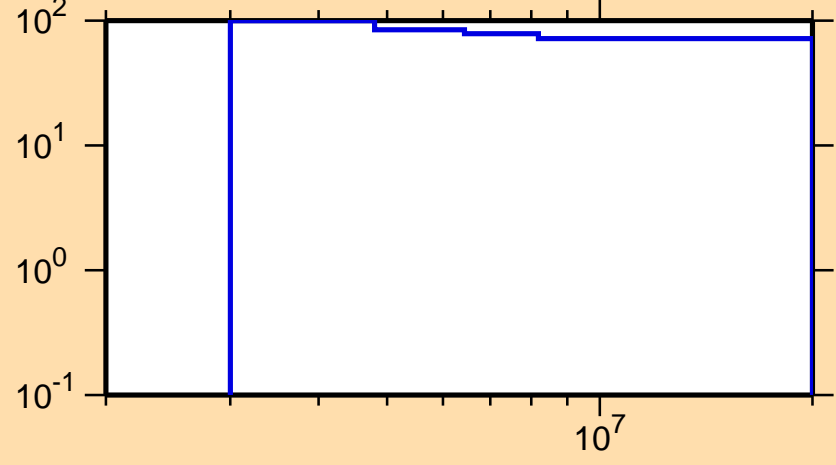
\Delta\sigma/\sigma vs. E for ^{252}\text{Bk}(n,2n)
