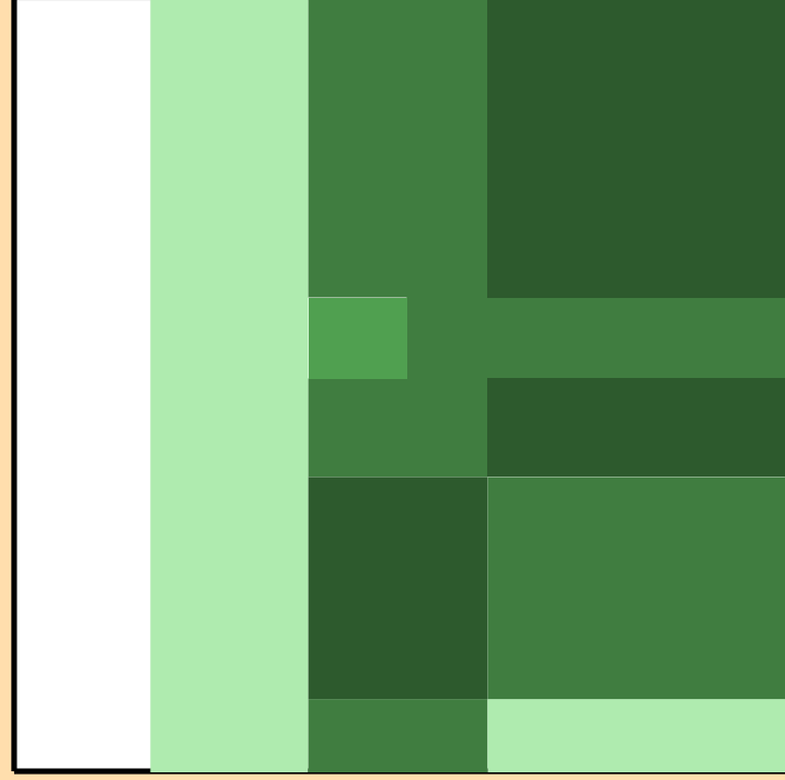
\Delta\sigma/\sigma vs. E for ^{252}\text{Bk}(n,2n)
