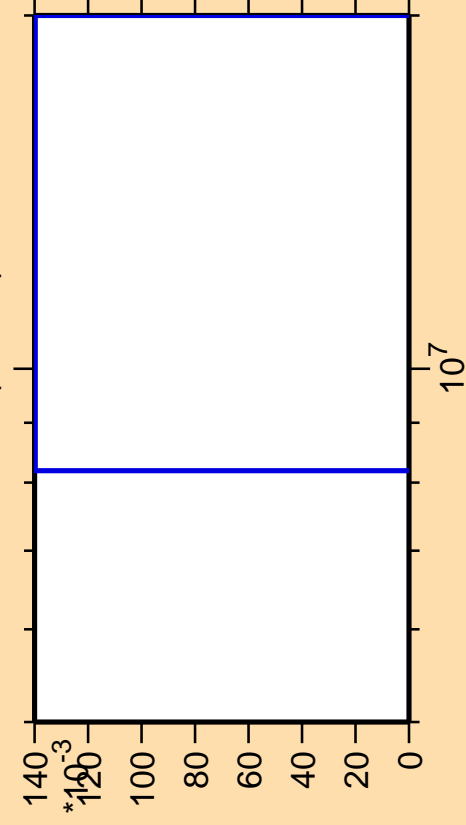
\Delta\sigma/\sigma vs. E for ^{252}\text{Bk} (mt 42)
