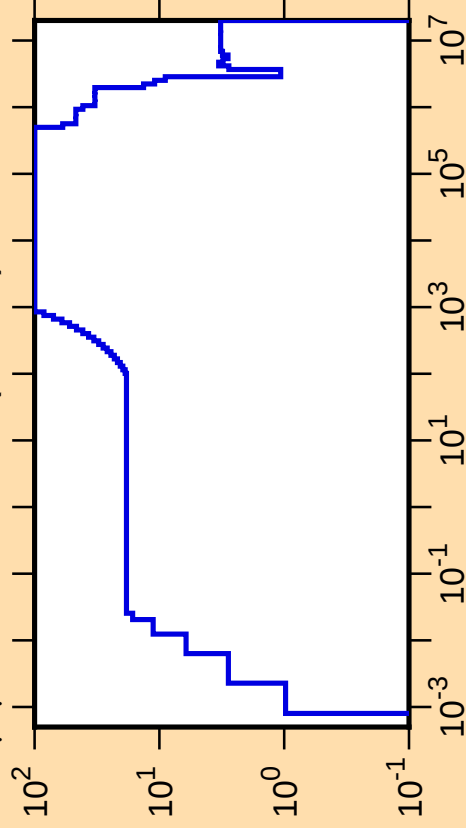
\Delta\mu/\mu vs. E for ^{253}\text{Bk}(\text{mt251})
