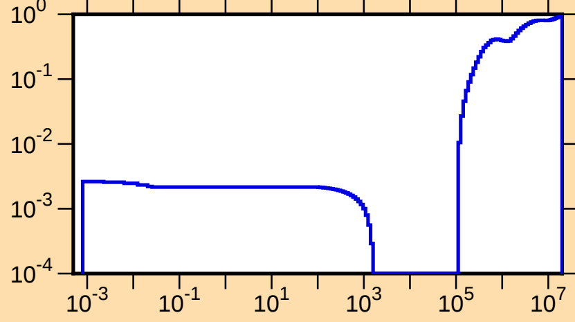
\mu vs. E for ^{253}\text{Bk}(\text{mt251})
