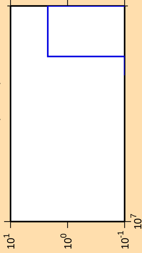
\Delta\sigma/\sigma vs. E for ^{253}\text{Bk}(n,\text{He}3)
