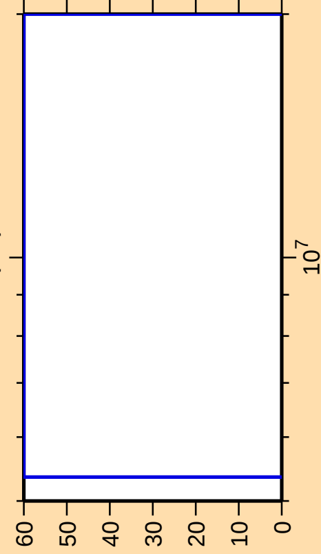
\Delta\sigma/\sigma vs. E for ^{253}\text{Bk}(n,f)
