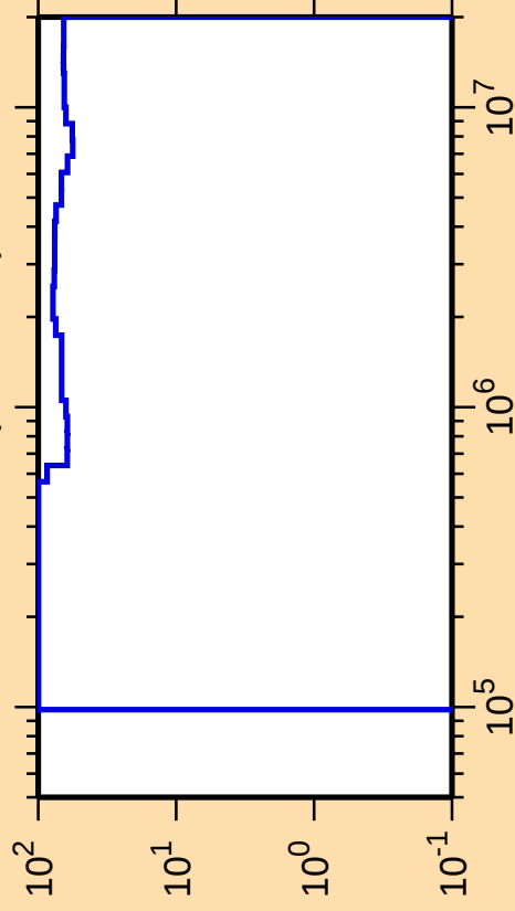
\Delta\sigma/\sigma vs. E for ^{253}\text{Bk}(n,\text{ncont.})
