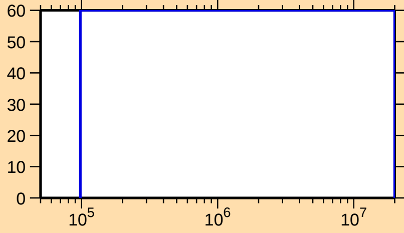
\Delta\sigma/\sigma vs. E for ^{253}\text{Bk}(n,\text{f})
