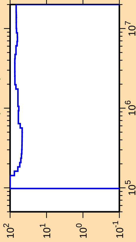
\Delta\sigma/\sigma vs. E for ^{253}\text{Bk}(n,\text{inel.})
