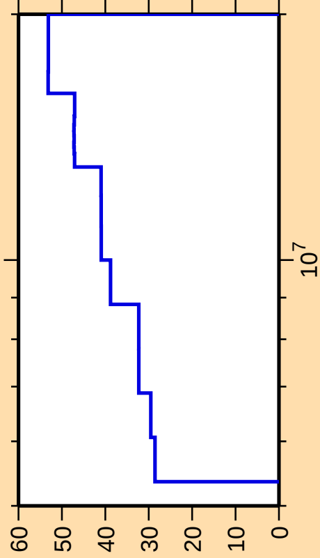
\Delta\sigma/\sigma vs. E for ^{253}\text{Bk}(n,n_1)
