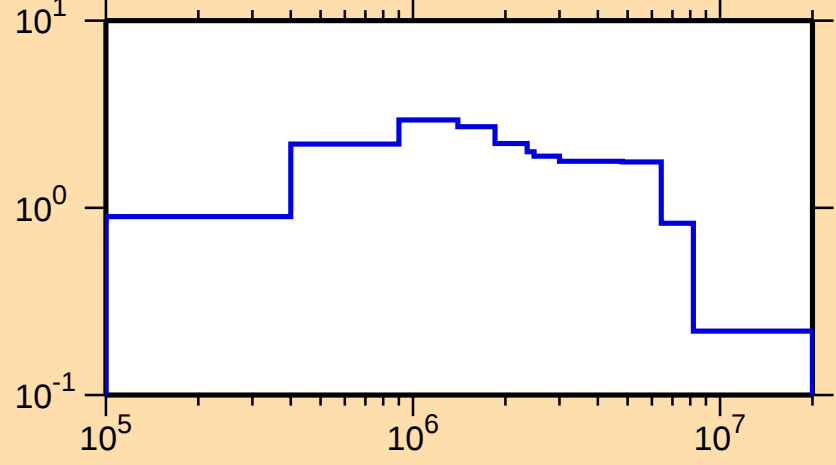
\sigma vs. E for ^{253}\text{Bk}(n,\text{inel.})
