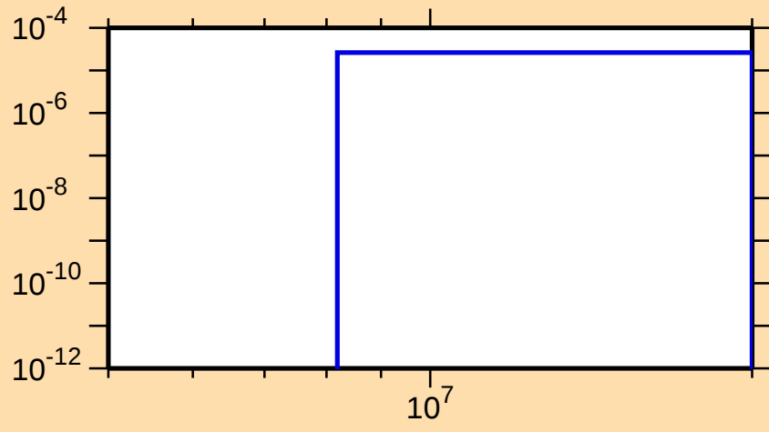
\sigma vs. E for ^{253}\text{Bk}(n,t)
