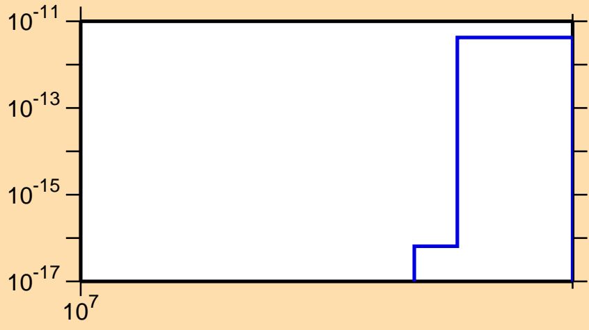
\sigma vs. E for ^{254}\text{Bk} (mt 11)
