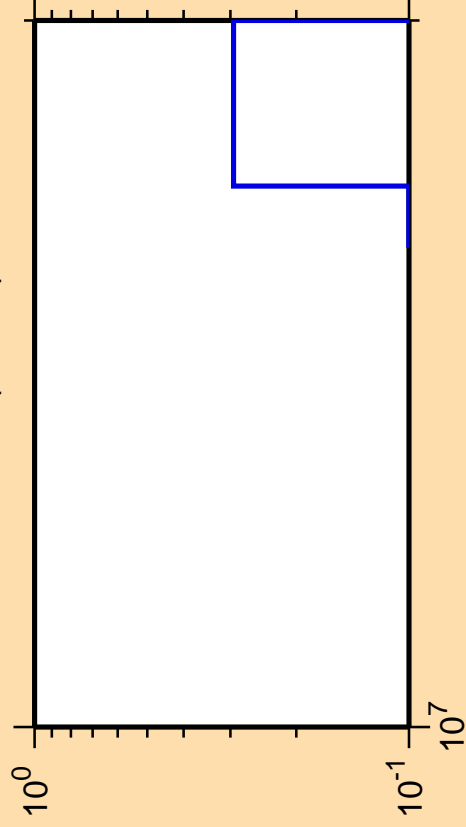
\Delta\sigma/\sigma vs. E for ^{254}\text{Bk} (mt 42)
