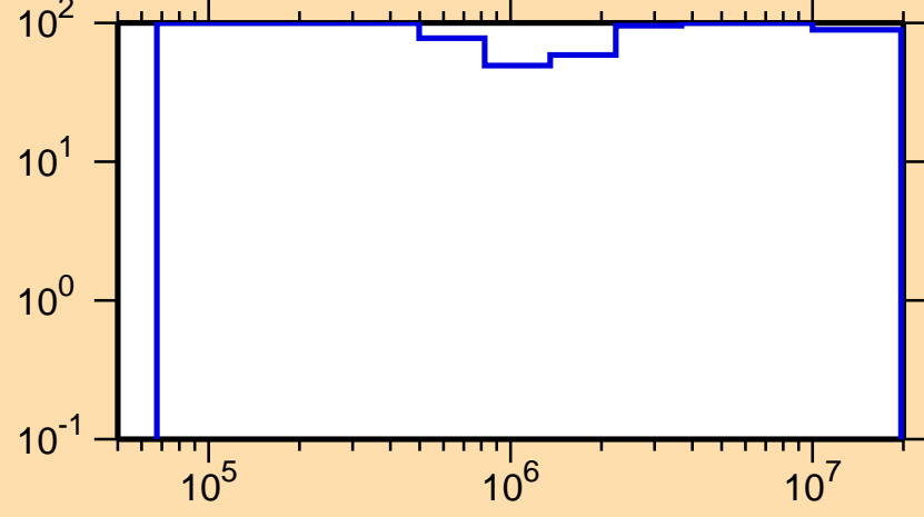
\Delta\sigma/\sigma vs. E for ^{254}\text{Bk}(n,\text{inel.})
