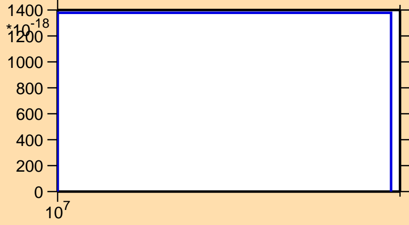
\sigma vs. E for ^{254}\text{Bk} (mt 42)
