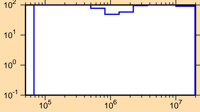
\Delta\sigma/\sigma vs. E for ^{254}\text{Bk}(n,n\text{cont.})
