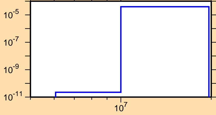
\sigma vs. E for ^{254}\text{Bk}(n,t)
