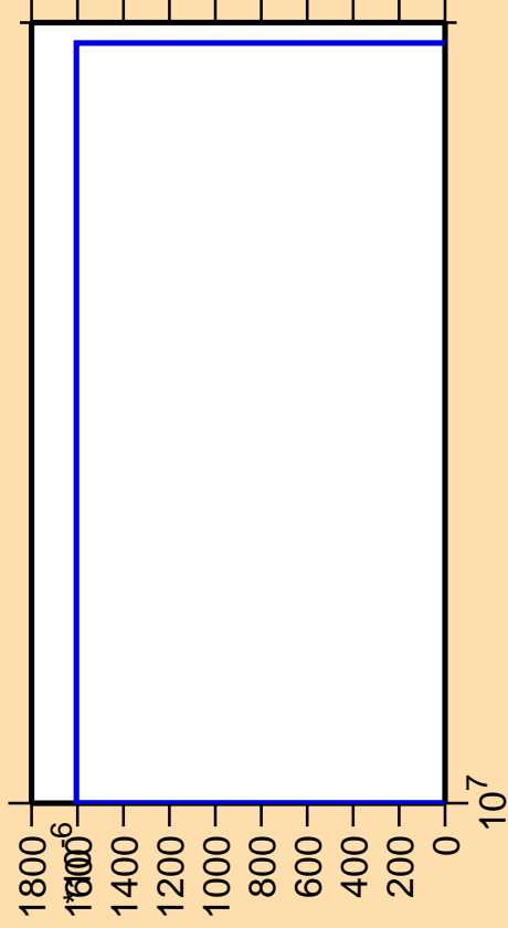
\Delta\sigma/\sigma vs. E for ^{254}\text{Bk} (mt 42)
