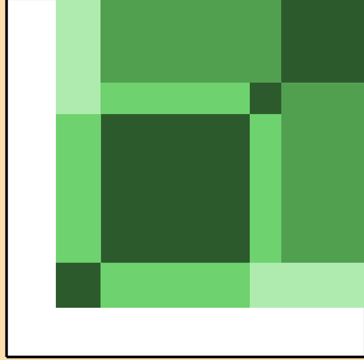
\sigma vs. E for ^{121}\text{Ce}(n,2n)
