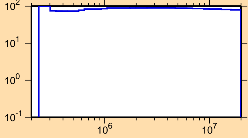
\Delta\sigma/\sigma vs. E for ^{121}\text{Ce}(n,n_1)
