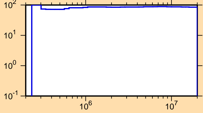
\Delta\sigma/\sigma vs. E for ^{121}\text{Ce}(n,\text{inel.})
