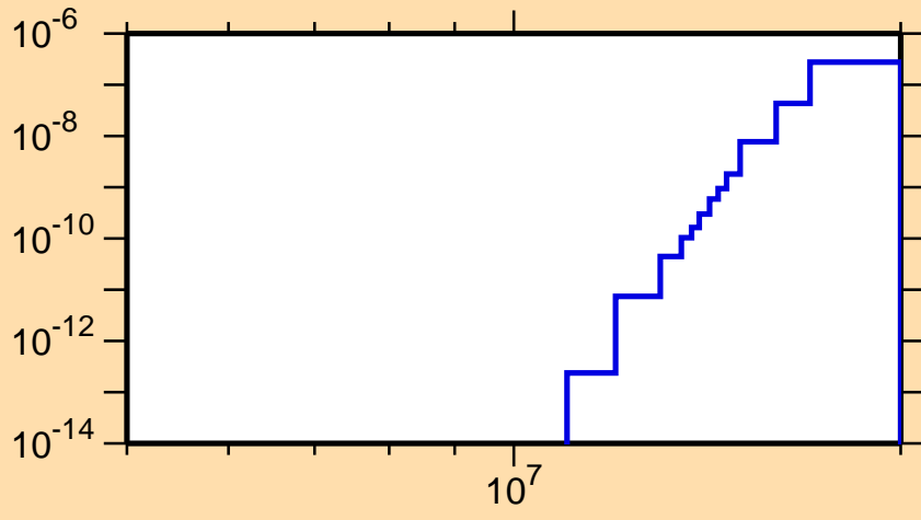
\sigma vs. E for ^{121}\text{Ce} (mt 34)
