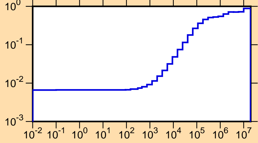
\mu vs. E for ^{121}\text{Ce}(\text{mt251})
