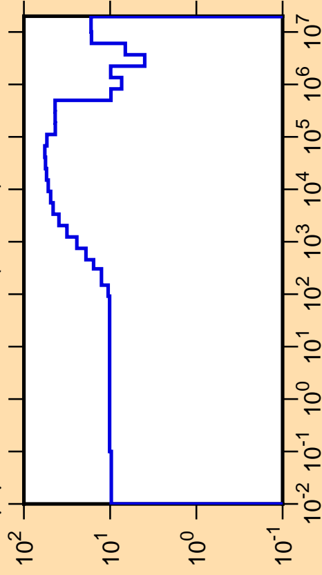
\Delta\mu/\mu vs. E for ^{121}\text{Ce}(\text{mt251})
