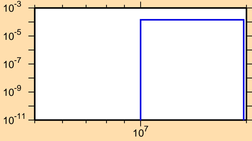
\sigma vs. E for ^{121}\text{Ce}(n,\text{pt})
