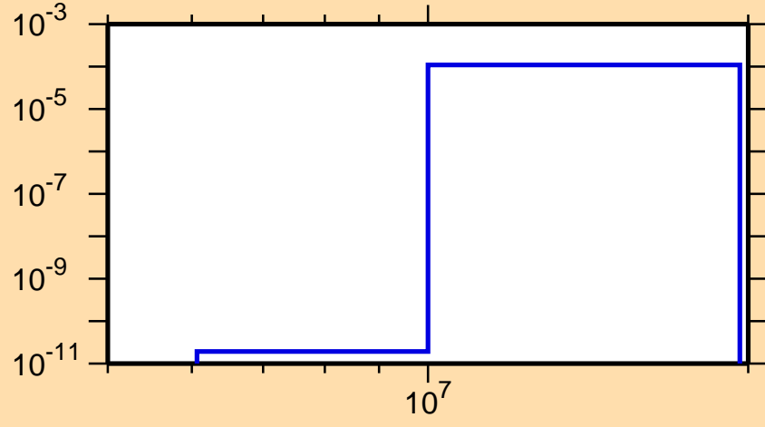
\sigma vs. E for ^{121}\text{Ce}(n,t)
