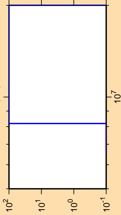
\Delta\sigma/\sigma vs. E for ^{121}\text{Ce}(n,t)
