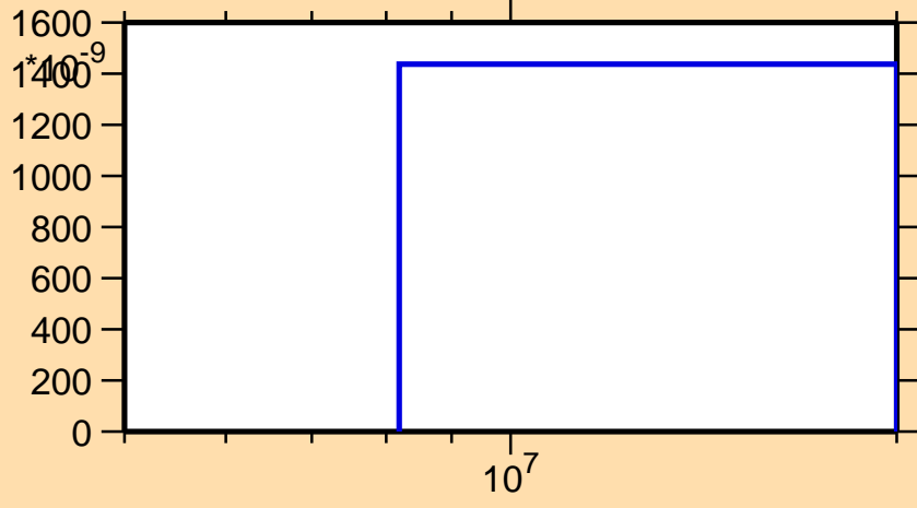
\sigma vs. E for ^{121}\text{Ce} (mt 45)
