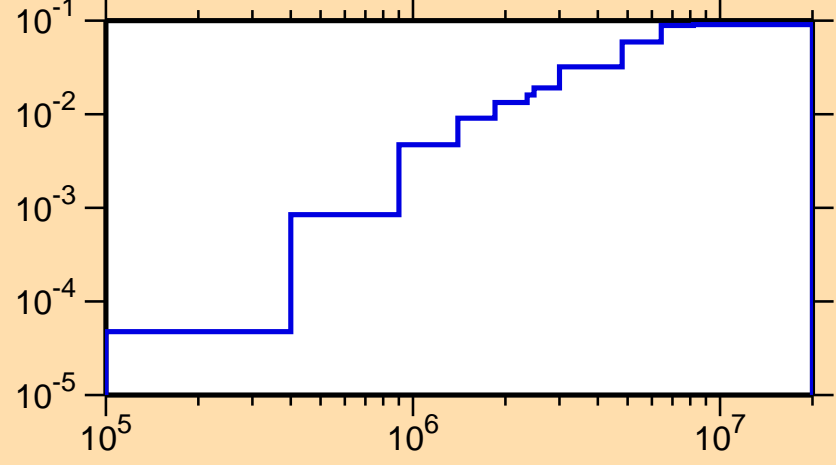
\sigma vs. E for ^{121}\text{Ce}(n,n\text{cont.})
