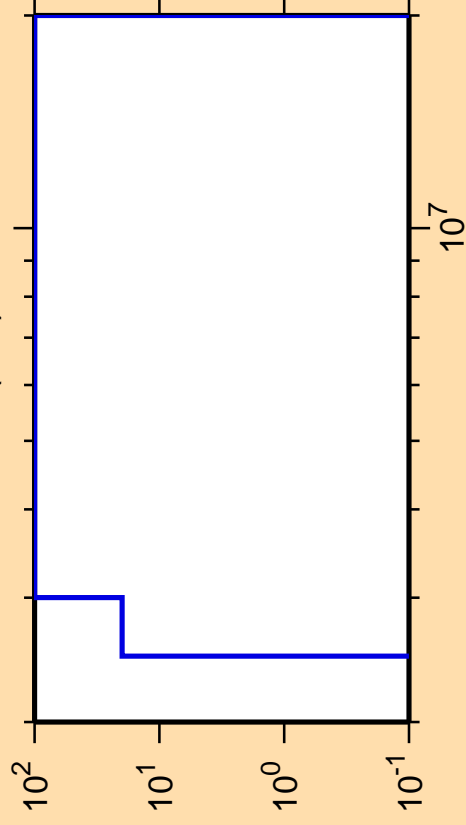
\Delta\sigma/\sigma vs. E for ^{121}\text{Ce}(n,d)
