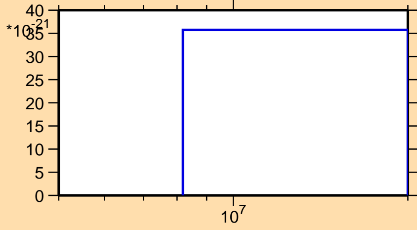
\sigma vs. E for ^{121}\text{Ce}(n,\text{nt})
