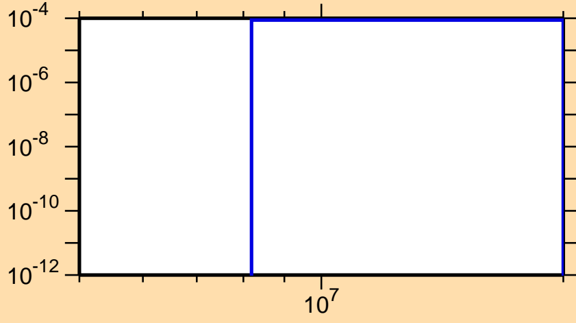
\sigma vs. E for ^{121}\text{Ce}(n,t)
