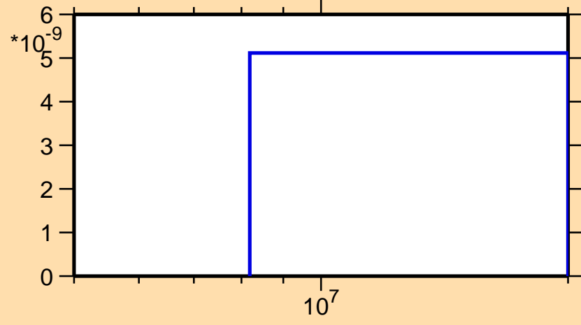
\sigma vs. E for ^{121}\text{Ce} (mt 34)
