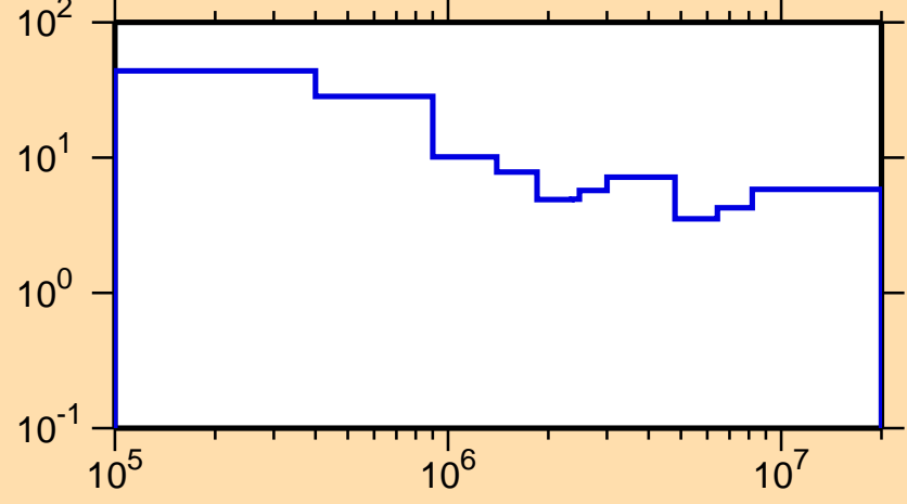
\Delta\sigma/\sigma vs. E for ^{121}\text{Ce}(n,\text{nonel.})
