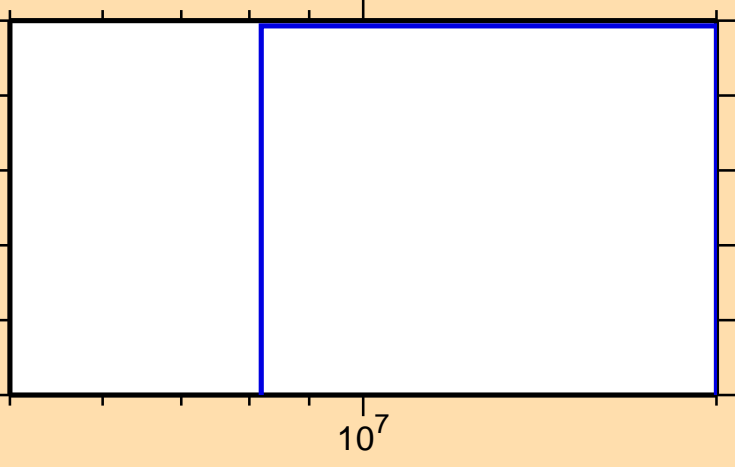
\sigma vs. E for ^{121}\text{Ce}(n,\text{nd})
