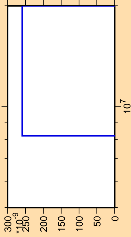
\Delta\sigma/\sigma vs. E for ^{121}\text{Ce}(n,\text{nt})
