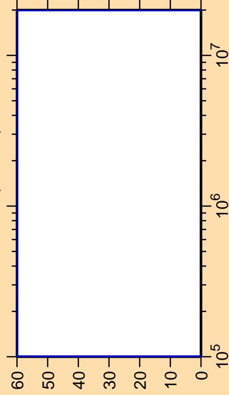
\Delta\sigma/\sigma vs. E for ^{121}\text{Ce}(n,\text{inel.})
