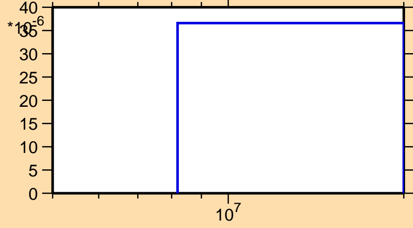
\sigma vs. E for ^{121}\text{Ce}(n,2n)
