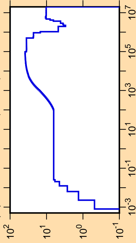
\Delta\mu/\mu vs. E for ^{122}\text{Ce}(\text{mt251})
