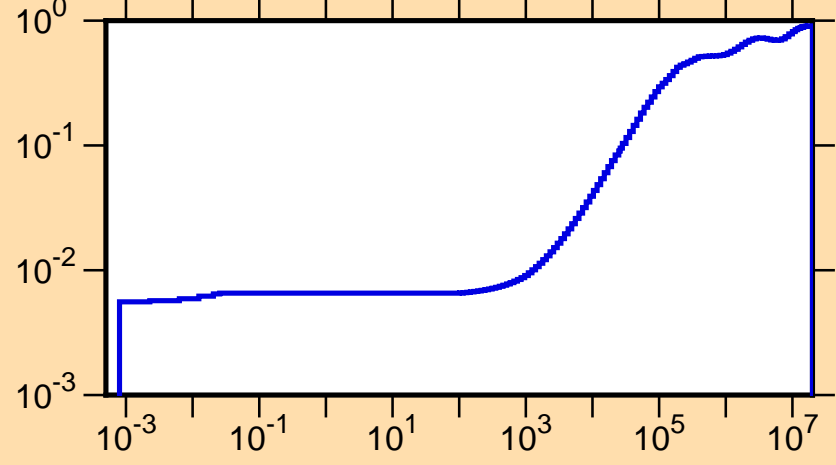
\mu vs. E for ^{122}\text{Ce}(\text{mt251})
