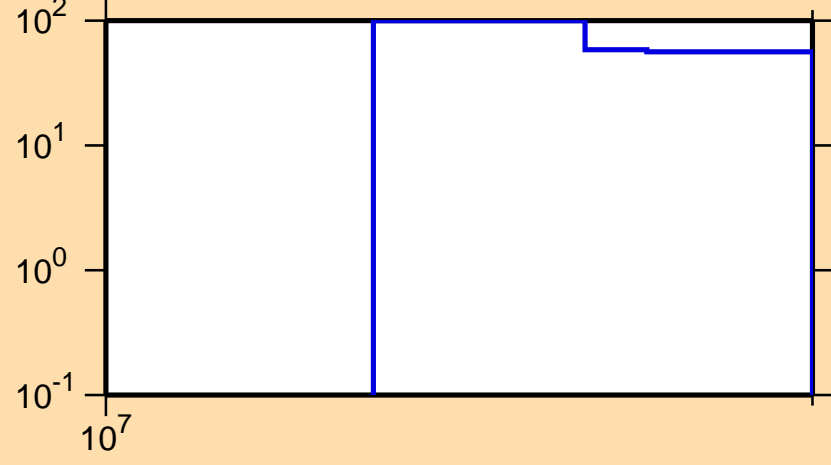
\Delta\sigma/\sigma vs. E for ^{122}\text{Ce}(n,2n)
