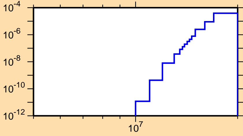
\sigma vs. E for ^{122}\text{Ce} (mt 45)
