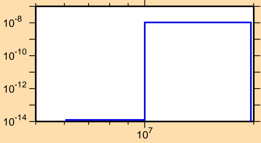
\sigma vs. E for ^{122}\text{Ce}(\text{mt117})
