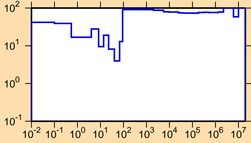
\Delta\sigma/\sigma vs. E for ^{122}\text{Ce}(n,\gamma)
