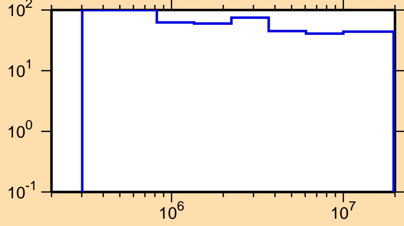
\Delta\sigma/\sigma vs. E for ^{122}\text{Ce}(n,n\text{cont.})
