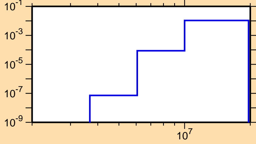
\sigma vs. E for ^{122}\text{Ce}(n,d)
