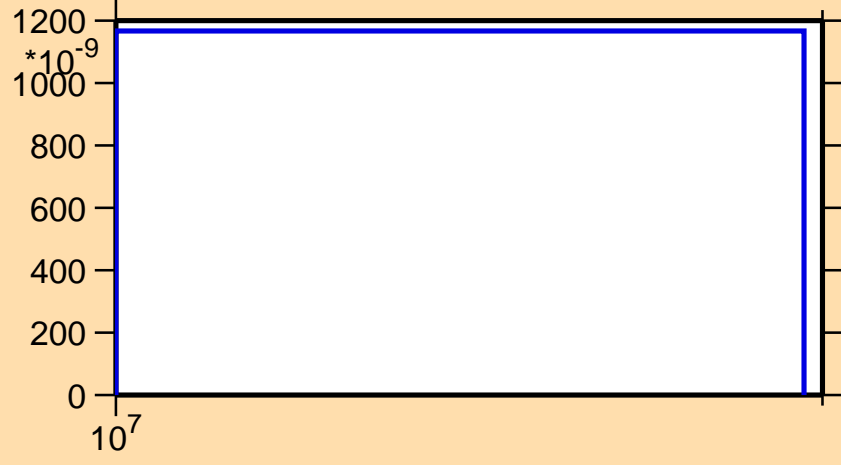
\sigma vs. E for ^{122}\text{Ce}(n,\text{pt})
