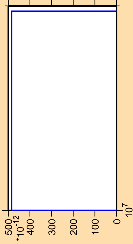
\Delta\sigma/\sigma vs. E for ^{122}\text{Ce}(n,nt)
