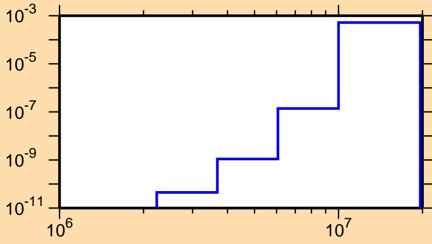
\sigma vs. E for ^{122}\text{Ce}(n,\text{He}3)
