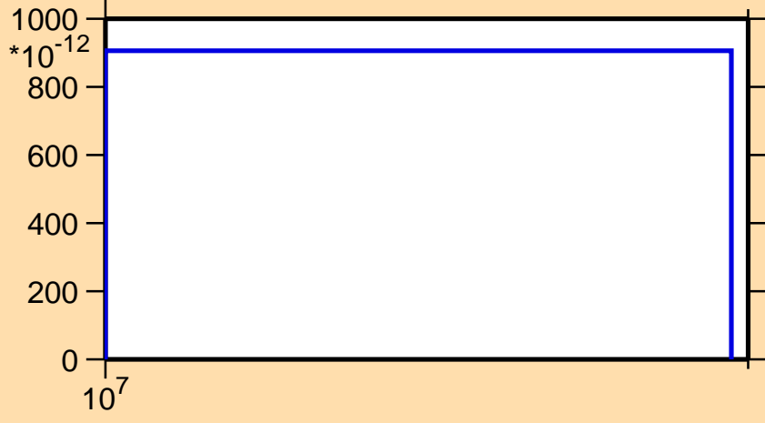
\sigma vs. E for ^{122}\text{Ce}(n,2np)
