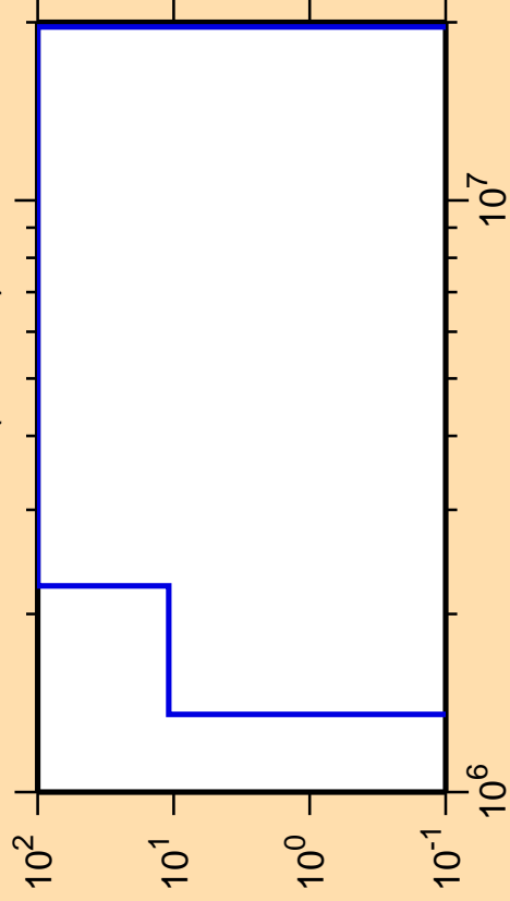
\Delta\sigma/\sigma vs. E for ^{122}\text{Ce}(n,\text{He}3)
