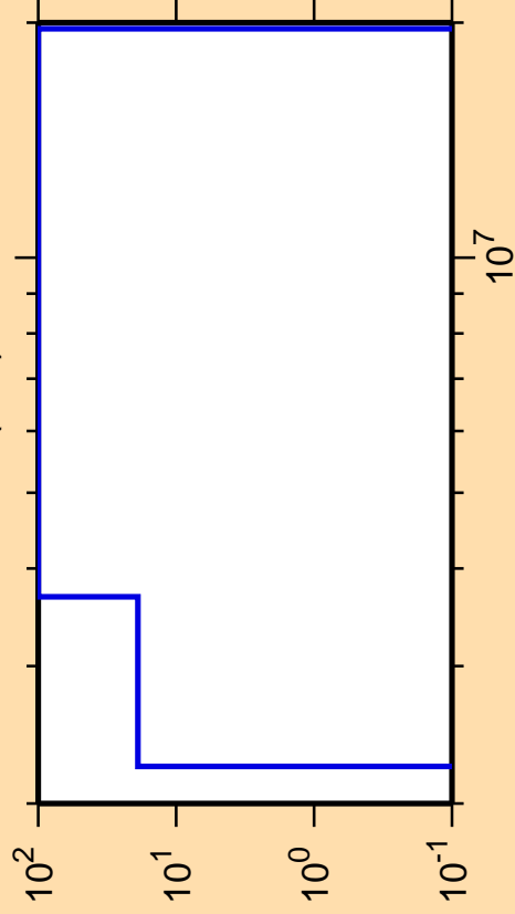
\Delta\sigma/\sigma vs. E for ^{122}\text{Ce}(n,d)
