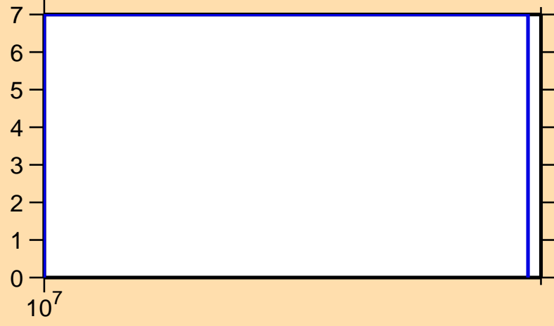
\Delta\sigma/\sigma vs. E for ^{122}\text{Ce}(n,\text{nonel.})
