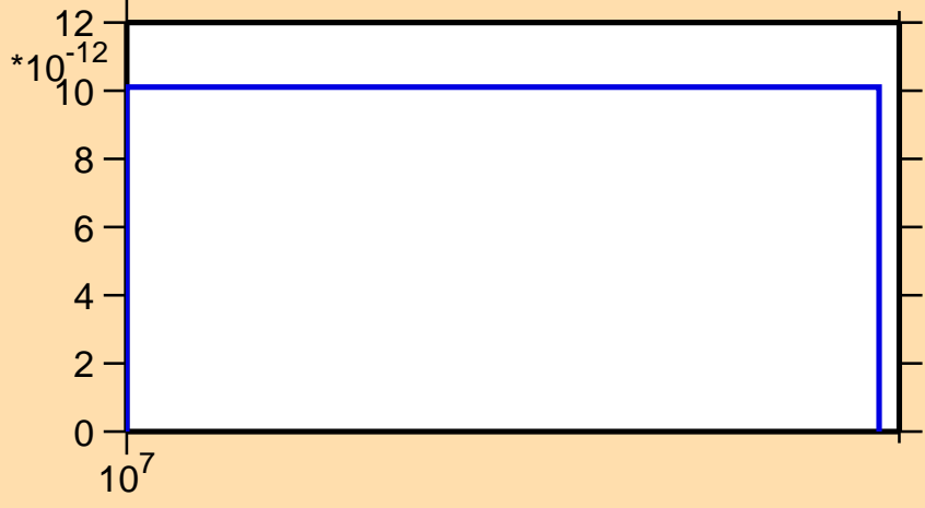
\sigma vs. E for ^{122}\text{Ce}(n,\text{nd})
