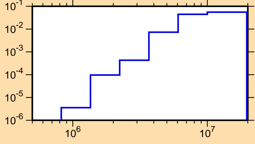
\sigma vs. E for ^{122}\text{Ce}(n,n\text{cont.})
