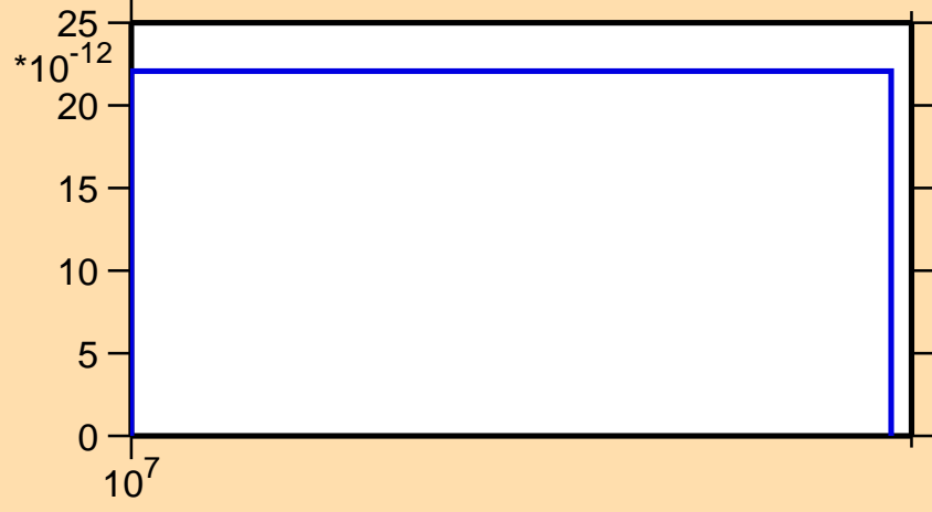
\sigma vs. E for ^{122}\text{Ce} (mt 34)
