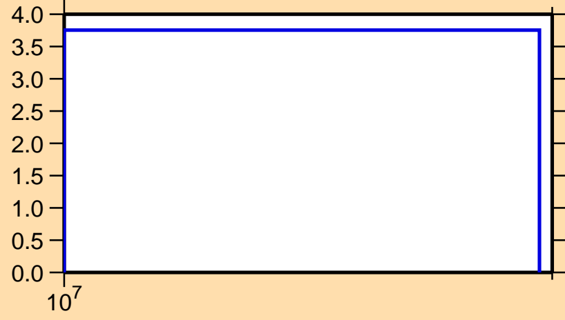
\Delta\sigma/\sigma vs. E for ^{122}\text{Ce}(n,\text{tot.})
