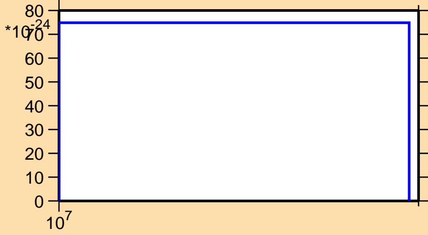
\sigma vs. E for ^{122}\text{Ce}(n,nt)
