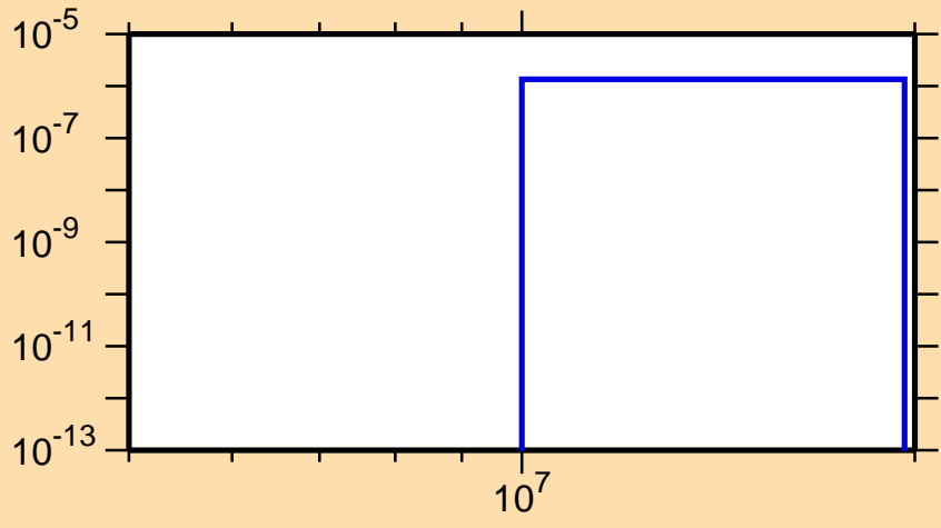
\sigma vs. E for ^{122}\text{Ce}(\text{mt } 45)
