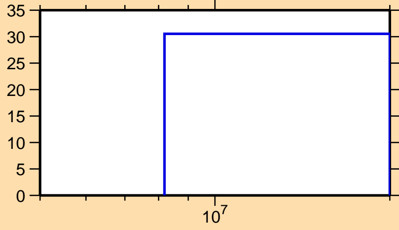
\Delta\sigma/\sigma vs. E for ^{122}\text{Ce}(n,\text{inel.})
