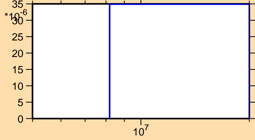
\sigma vs. E for ^{122}\text{Ce}(n,t)
