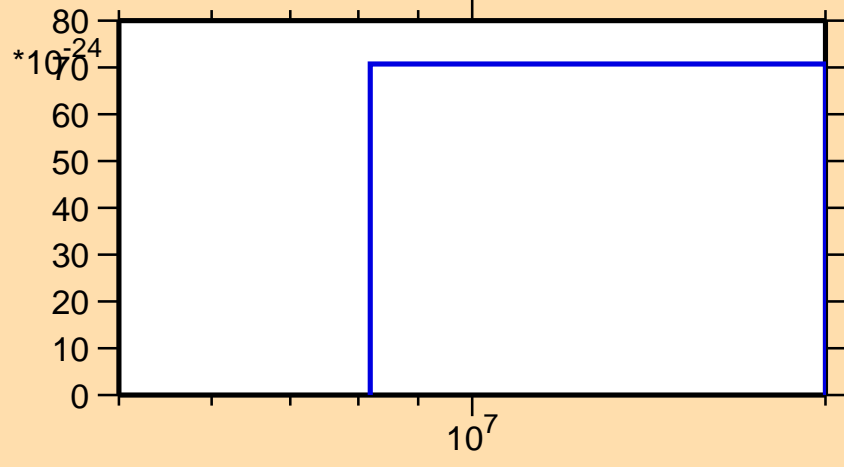
\sigma vs. E for ^{122}\text{Ce}(n,\text{nt})
