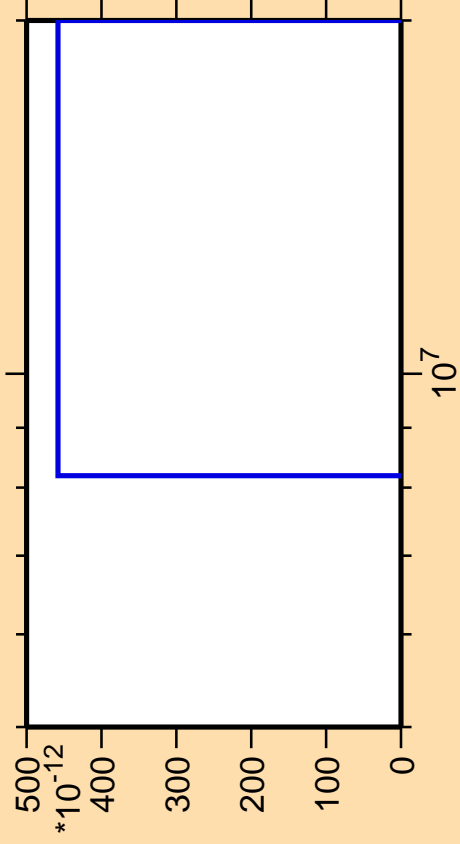
\Delta\sigma/\sigma vs. E for ^{122}\text{Ce}(n,\text{nt})
