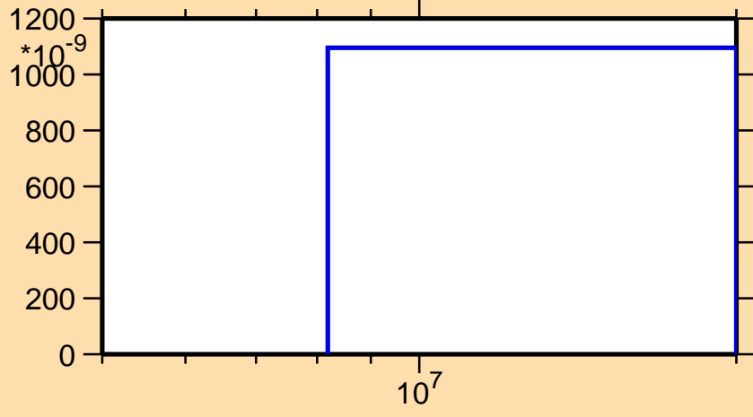
\sigma vs. E for ^{122}\text{Ce} (mt 45)
