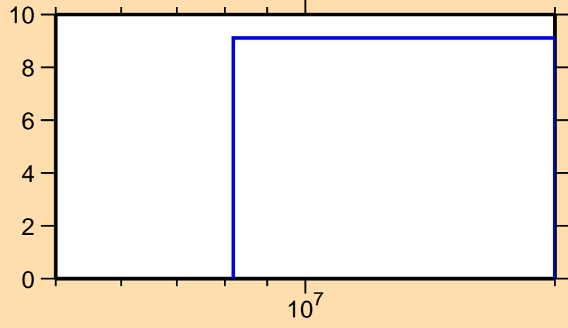
\Delta\sigma/\sigma vs. E for ^{122}\text{Ce}(n,\text{el.})
