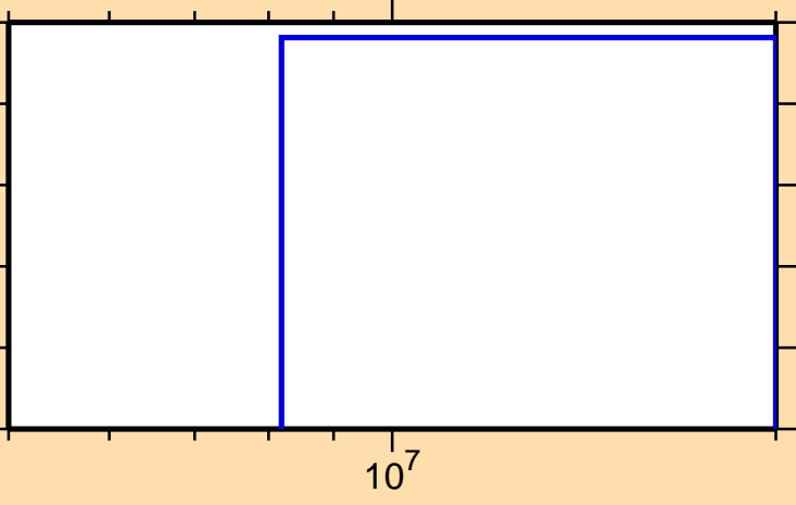
\sigma vs. E for ^{122}\text{Ce}(n,\text{pt})
