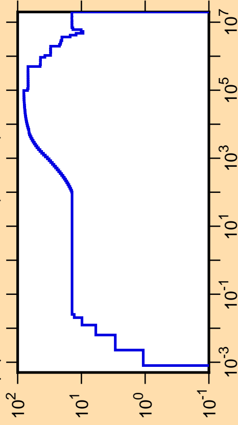
\Delta\mu/\mu vs. E for ^{123}\text{Ce}(\text{mt251})
