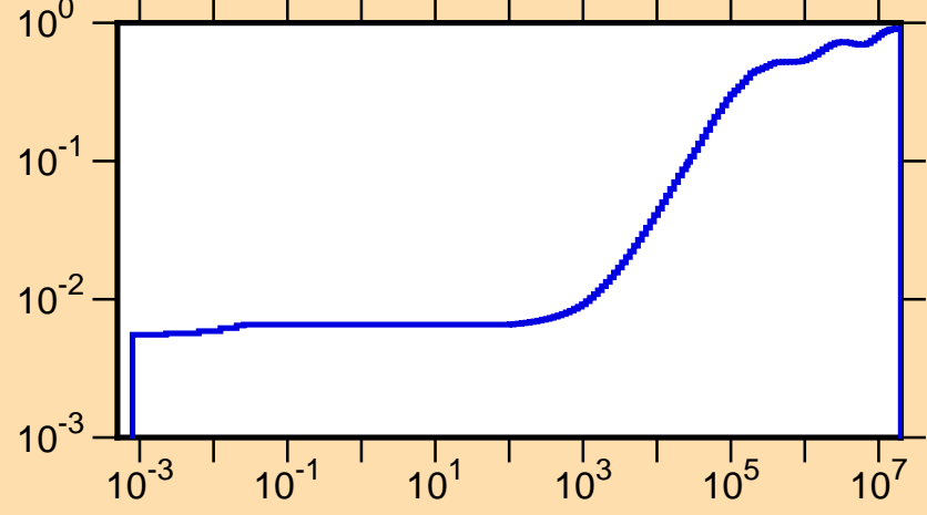
\mu vs. E for ^{123}\text{Ce}(\text{mt251})
