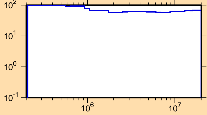
\Delta\sigma/\sigma vs. E for ^{123}\text{Ce}(n,n_1)
