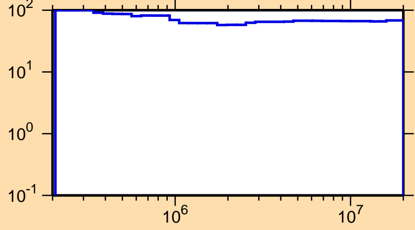
\Delta\sigma/\sigma vs. E for ^{123}\text{Ce}(n,\text{inel.})
