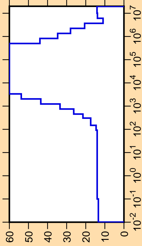
\Delta\mu/\mu vs. E for ^{123}\text{Ce}(\text{mt251})
