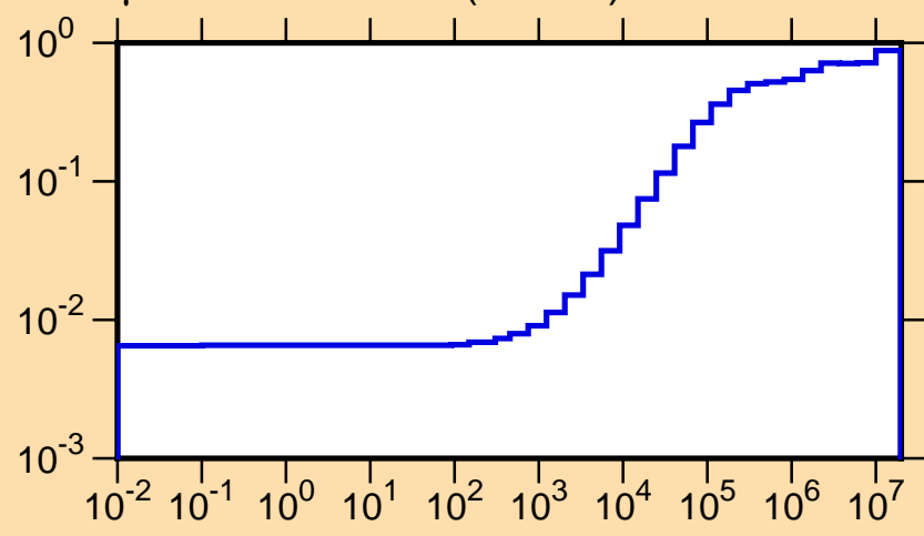
\mu vs. E for ^{123}\text{Ce}(\text{mt251})
