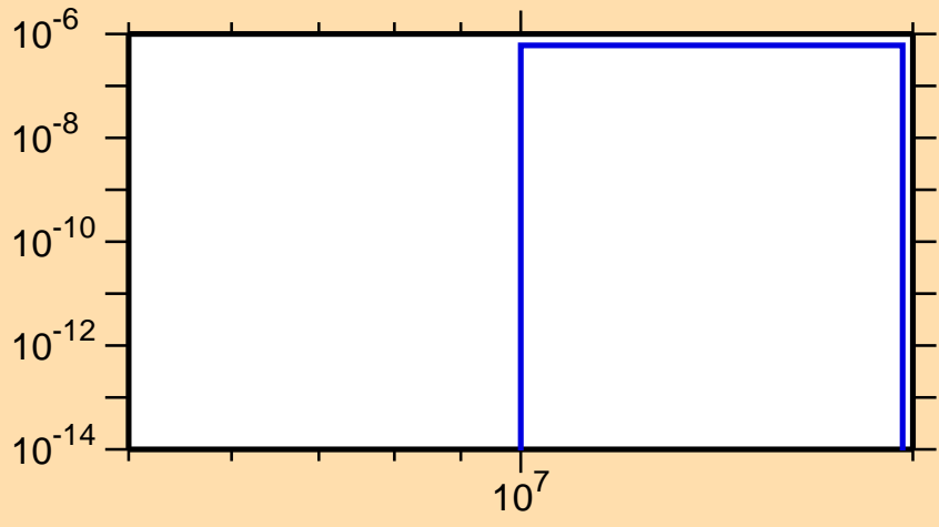
\sigma vs. E for ^{123}\text{Ce}(\text{mt } 45)
