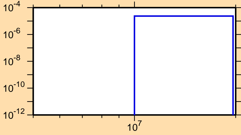
\sigma vs. E for ^{123}\text{Ce}(n,\text{pt})
