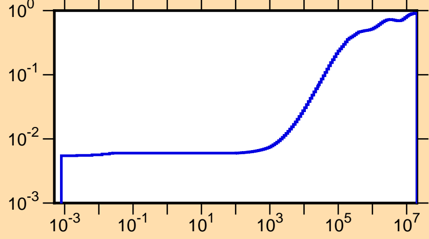
\mu vs. E for ^{124}\text{Ce}(\text{mt251})
