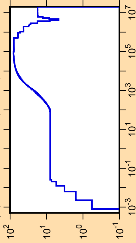
\Delta\mu/\mu vs. E for ^{124}\text{Ce}(\text{mt251})
